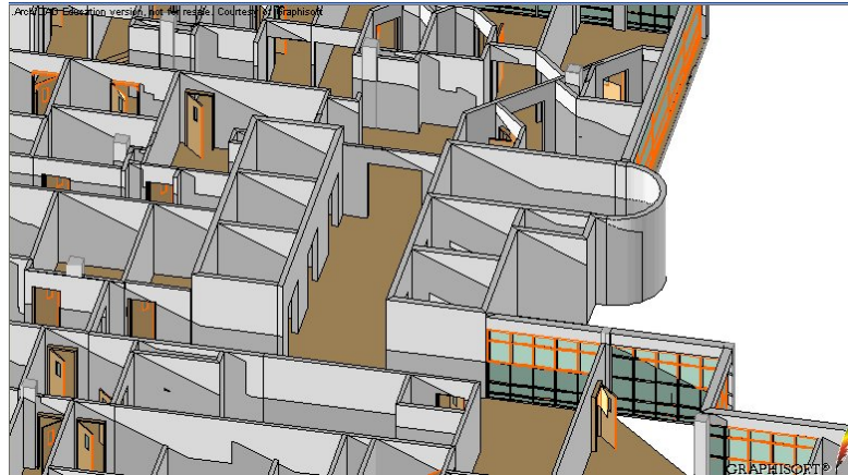
Figure 5. 3D view of vertical transportation area (Lifts and stairs) at Building 10, Royal Prince Alfred Hospital.
