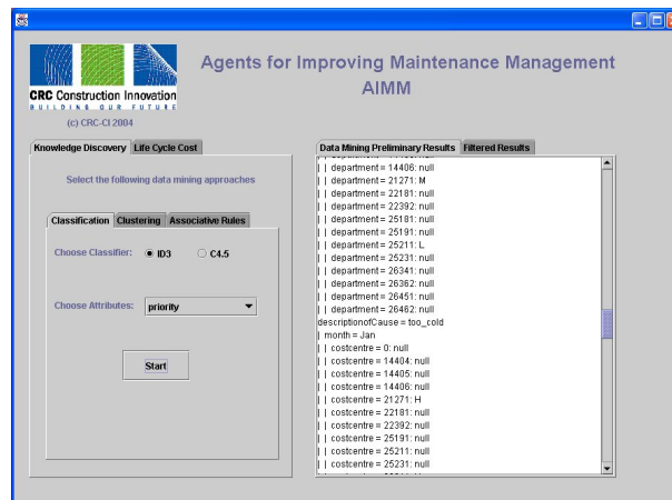
Figure 14. Preliminary results of applying the ID3 with the "Priority" attribute on AHU maintenance data.
