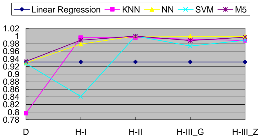
Figure .1: Correlation Coefficient of KNN, NN, SVM & M5
