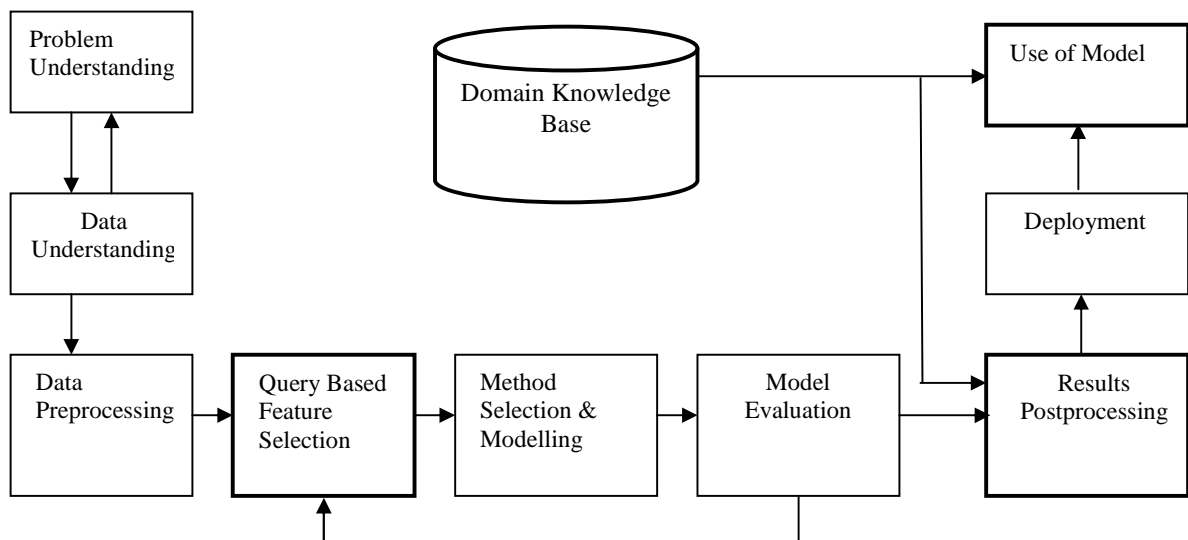
Figure 1. Query Based Learning System
