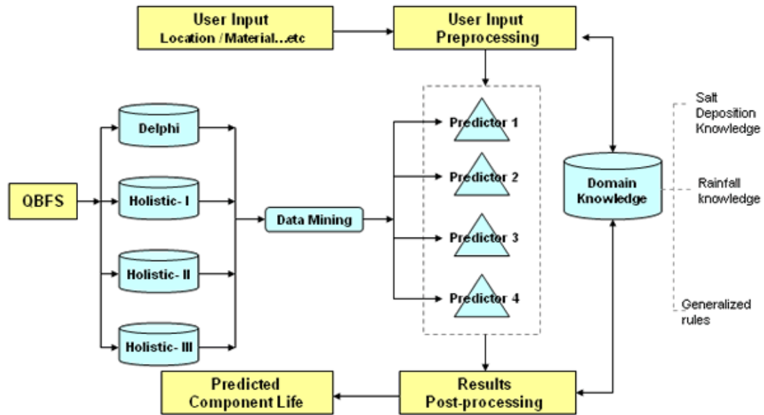
Figure 1. Overview of System
