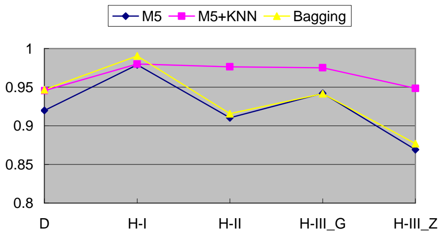
Figure 3. Correlation Coefficient of M5, M5+KNN and Bagging (D=Delphi, H-I=Holistic-I, H-II= Holistic-II, H-III_G=Holistic-III for Galvanized Steel, H-III_Z=Holistic-III for Zinalume)
