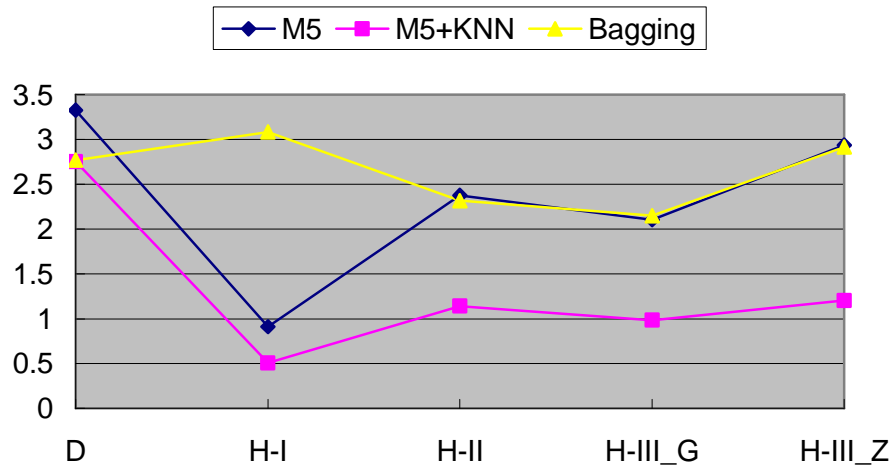
Figure 4. Mean Absolute Error of M5, M5+KNN and Bagging, (D=Delphi, H-I=Holistic-I, H-II= Holistic-II, H-III_G=Holistic-III for Galvanized Steel, H-III_Z=Holistic-III for Zinalume)
