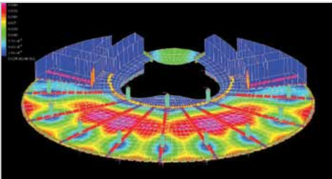
Analysis and design of post-tensioned and reinforced concrete floor systems using Ram Concept®
