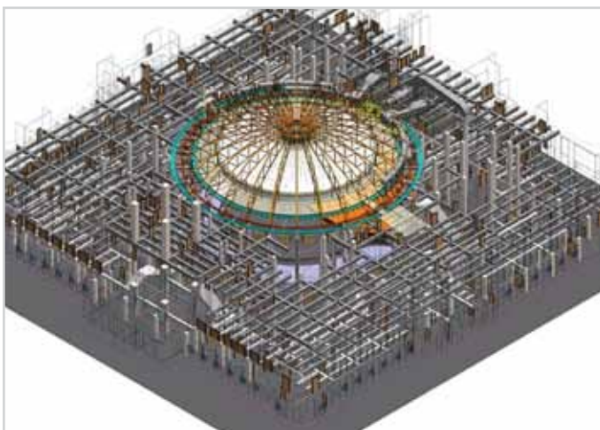
City Hall – BIM showing the structural layer
