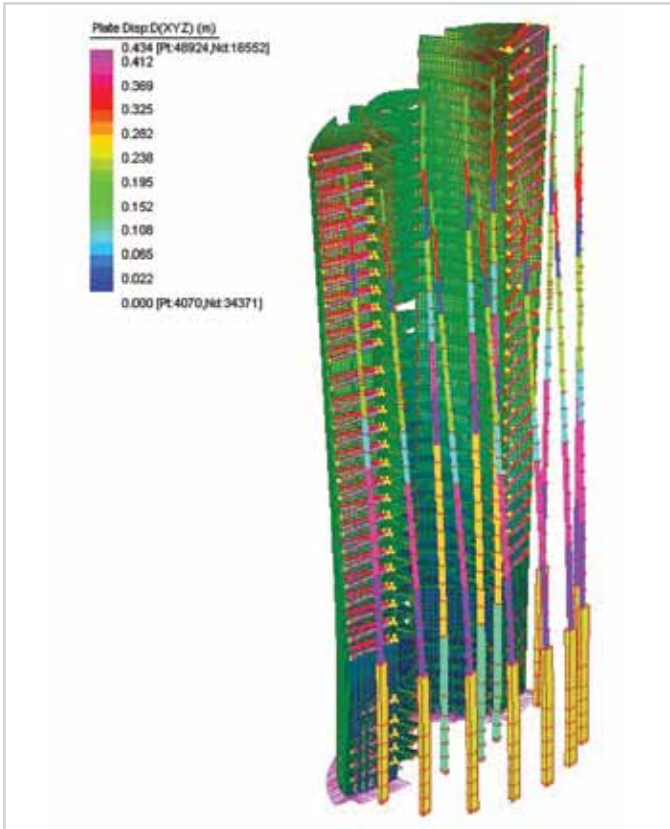
Finite element analysis of the structural design using Strand7®
