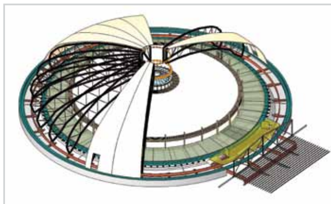
City Hall – 3D model of the central dome showing layers of existing and proposed building fabric
