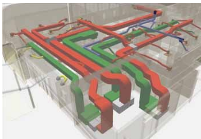
North Lakes Police Station – mechanical clash detection
