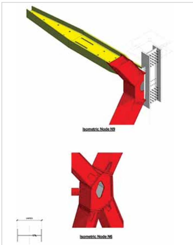
Structural meganode Image courtesy Arup
