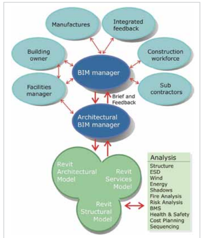
Proposed BIM conceptual model for 1 Bligh Street project
