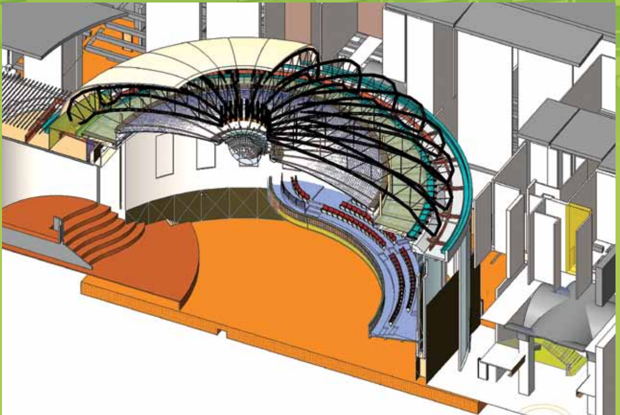
Brisbane City Hall Auditorium roof model
