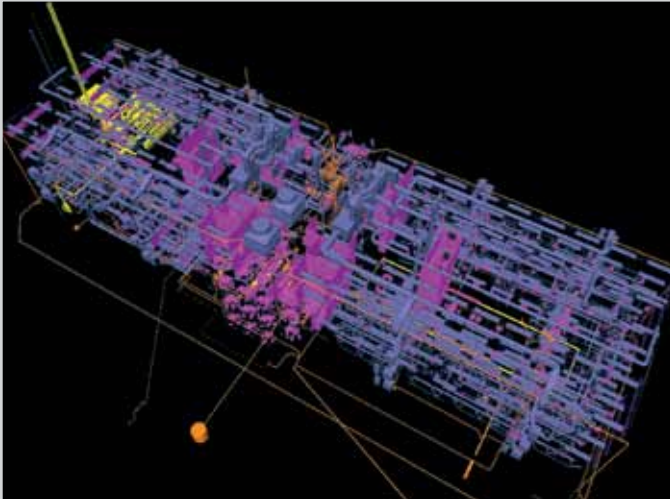
JCC Zillmere – clash detection models (continued)
