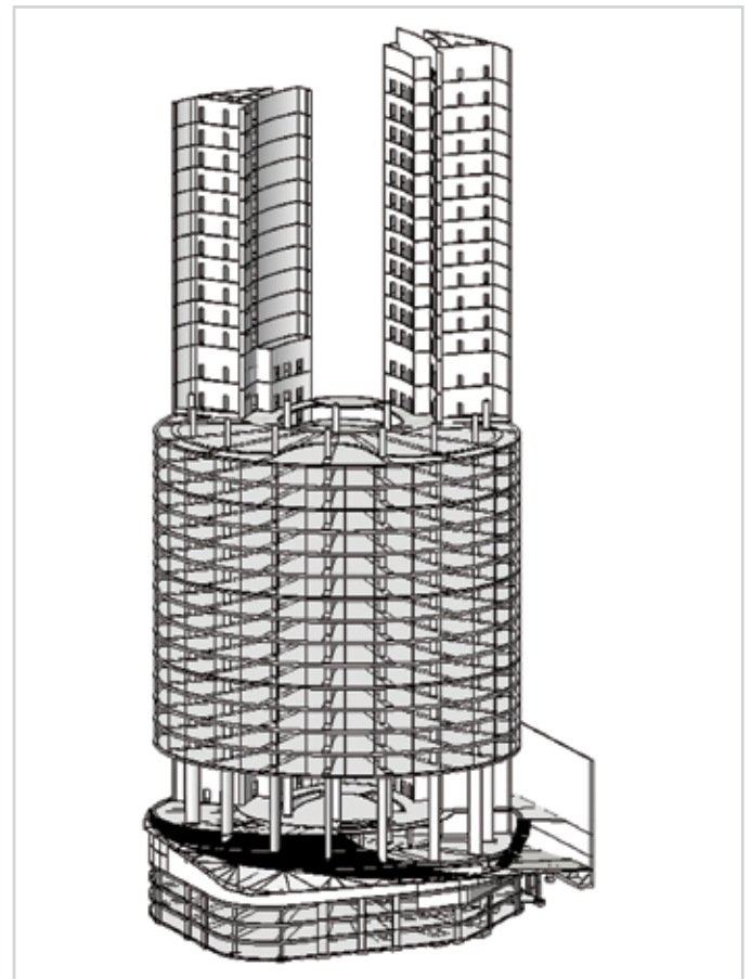
3D view of the structural model in Revit® Structures
