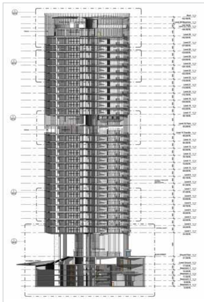
Section of 1 Bligh Street done in Revit® Image courtesy Architectus and Ingenhoven Architects
