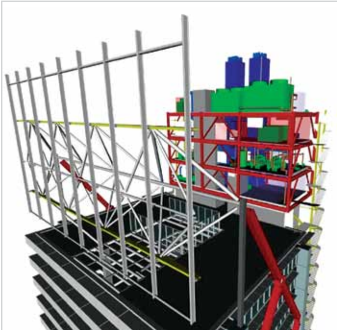
Revit® SMEP Image courtesy Arup
