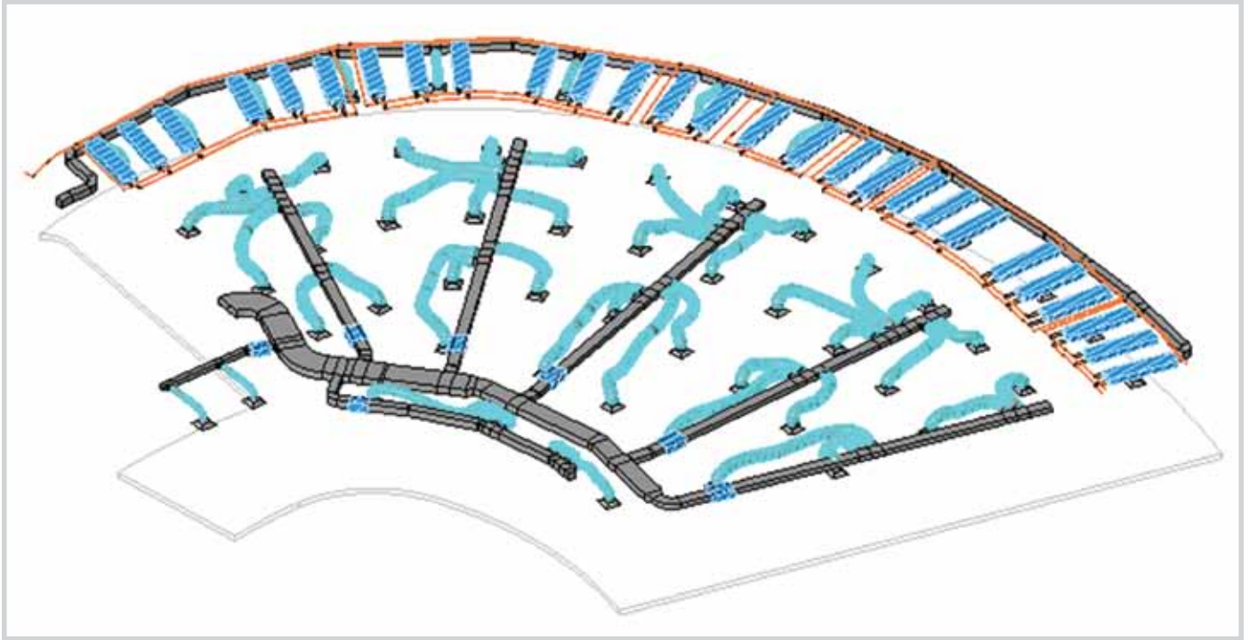
Mechanical services of a typical floor using Revit® Services
