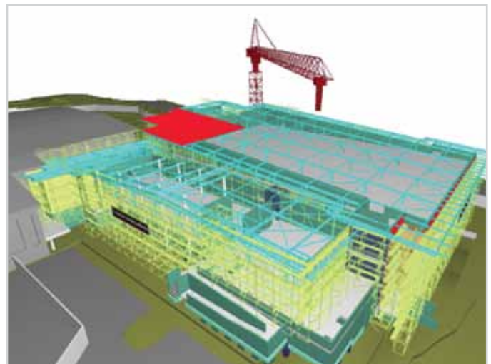
State Archives Extension Project – 4D model view
