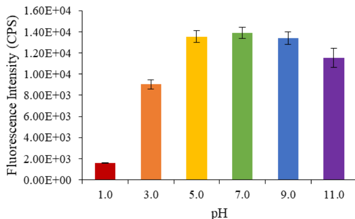
Figure 5.6: GQDs-hMSNs with changing pH (maleate pH 1.0, citrate 3.0-5.0, HEPES 7.0, CHES 9.0, CAPS 11.0) of the GQDs-hMSNs (36 \mu\text{g}/\text{mL} ). The same trend was observed for GQDs, where quantum dots quench in pH 1.0 but remain steady in the neutral pHs.
