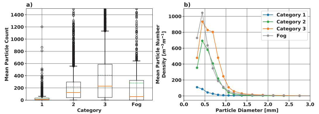
Figure 8. (a) Boxplots of mean particle counts from the Parsivel 2 for each category based on the 5-min + MET algorithm. The orange solid and green dashed lines represent the median and mean of the distributions, respectively. (b) Mean particle number density distributions from Parsivel 2 separated by category.
