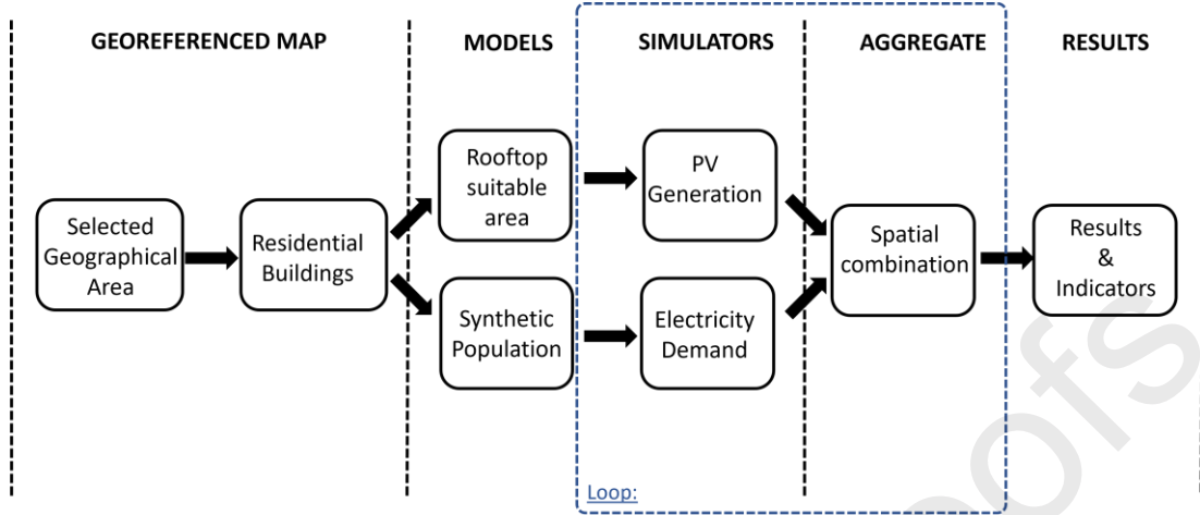
Fig. 2. Orchestrator work-flow.
