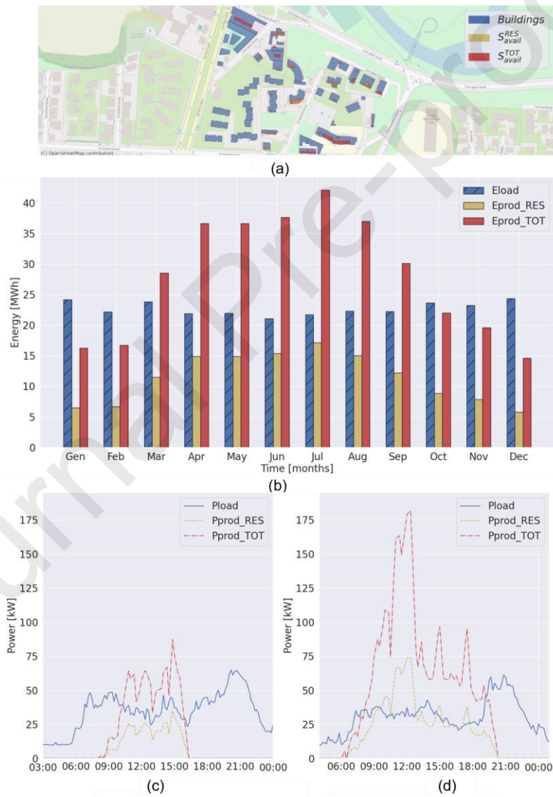
Fig. 4. Summary results for the census tract in Parella: (a) A georeferenced representation of the available building and rooftop surfaces for Scenario RES ( S_{avail}^{RES} ) and for Scenario TOT ( S_{avail}^{TOT} ); (b) a histogram of the monthly consumed energy ( E_{load} ), monthly produced energy with Scenario RES
