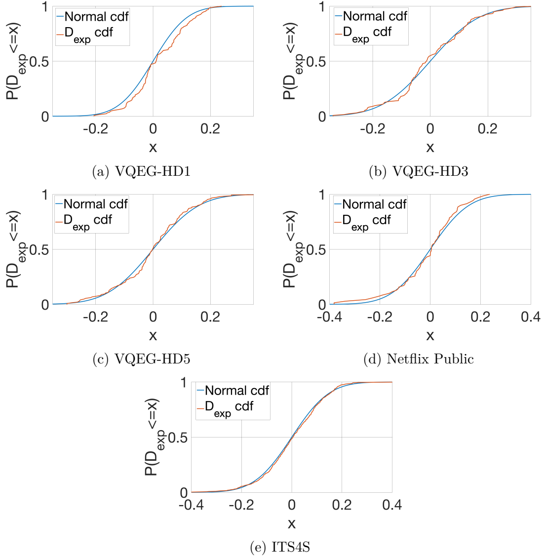
Figure 3.4: Comparison between the empirical cumulative distribution function (orange curve) of D_{exp} and that of a Gaussian random variable having 0 as mean and similar standard deviation with D_{exp} (blue curve). The analysis was done on five different datasets. The fact that the empirical cumulative distribution of D_{exp} , for each dataset, so closely approximates the cumulative distribution of the related Gaussian distribution shows that D_{exp} can also be considered distributed according to this Gaussian distribution.
