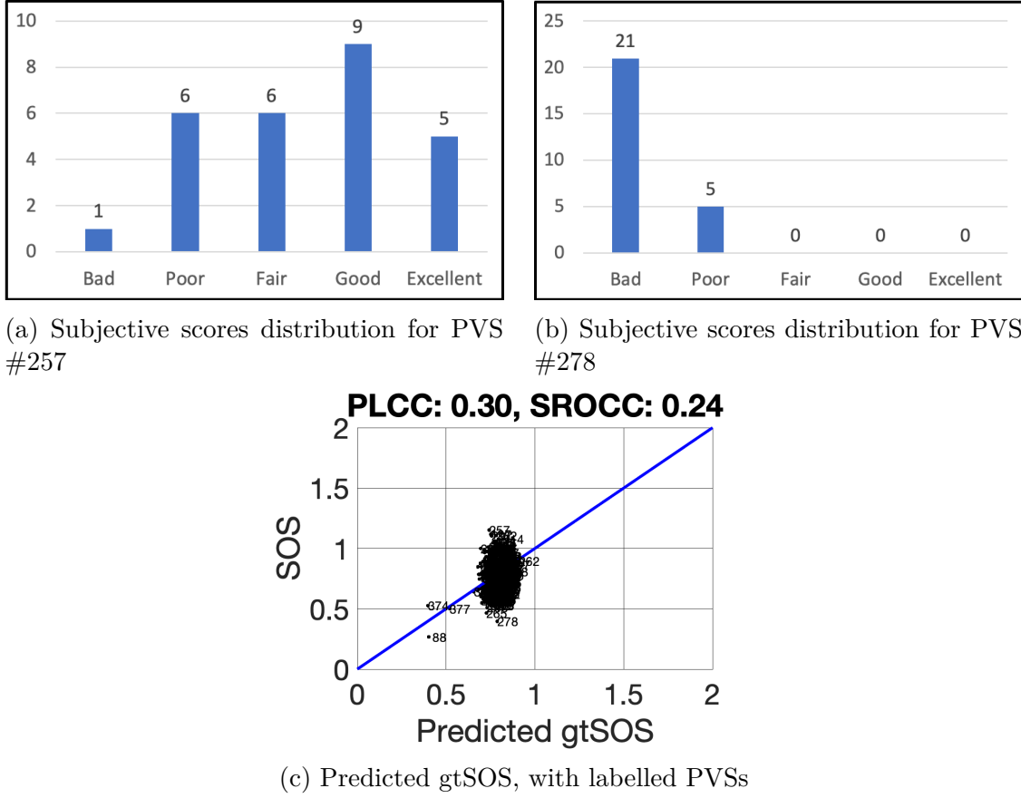
Figure 3.11: Analyzing the ITS4S dataset. The value of D_{exp} is large for PVSs #257 and #278. The opinion scores for PVS #257 are almost uniformly distributed over the quality scale; this highlights the peculiar nature of the subjective evaluation of such a PVS. On the other hand, the analysis indicated that the low SOS value of the PVS #278 may not be a reliable estimation of its ability to generate diversity among viewers' ratings.
