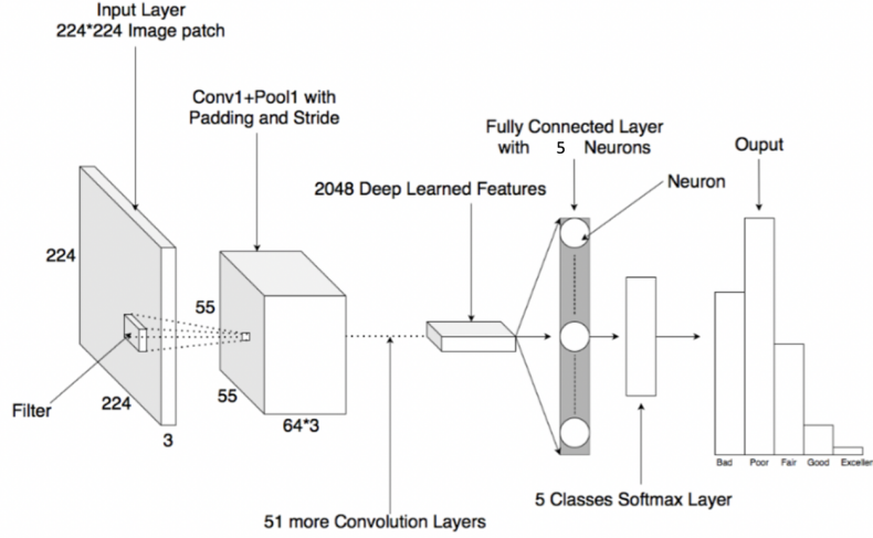
Figure 6.3: Architecture of the JPEGResNet50 as well as of the AIOs. This network receives as an input a 224 \times 224 color image and provides as an output an estimation of the probability that an average viewer would choose any of the five options of the ACR scale.
