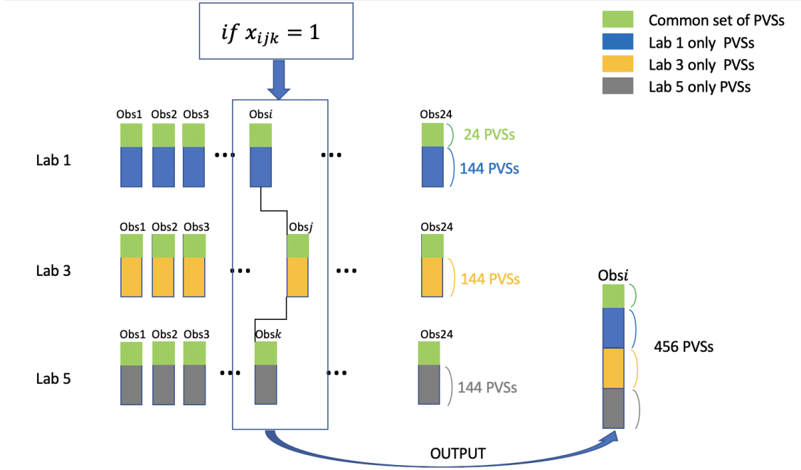
Figure 5.3: Proposed data augmentation approach. Each viewer of the Lab 1 was put together with a viewer of the Lab 3 and a viewer of Lab 5 based on the solution of the optimization problem. This yielded 24 viewers that were considered to have rated 456 PVSs instead of 168.
