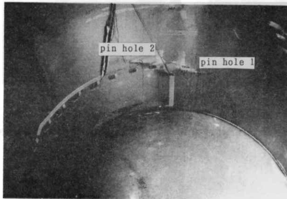
写真 25 脚部ダイヤモンドタイプ座屈の内面 Photo 25 Inside Appearance of Diamond Type Buckling in Footholds of Vessel
