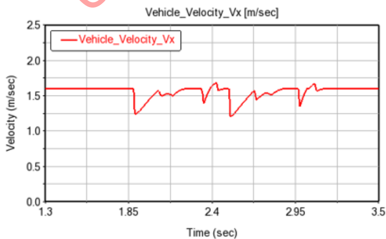
Fig. 4. Velocity of robot in the X direction
