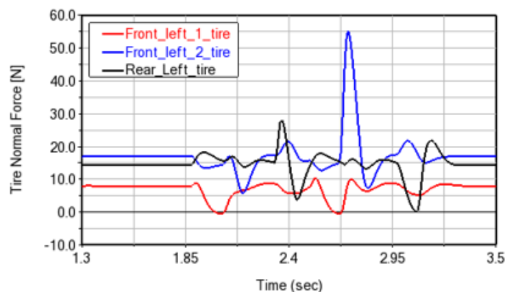
Fig. 6. Normal forces on wheels
