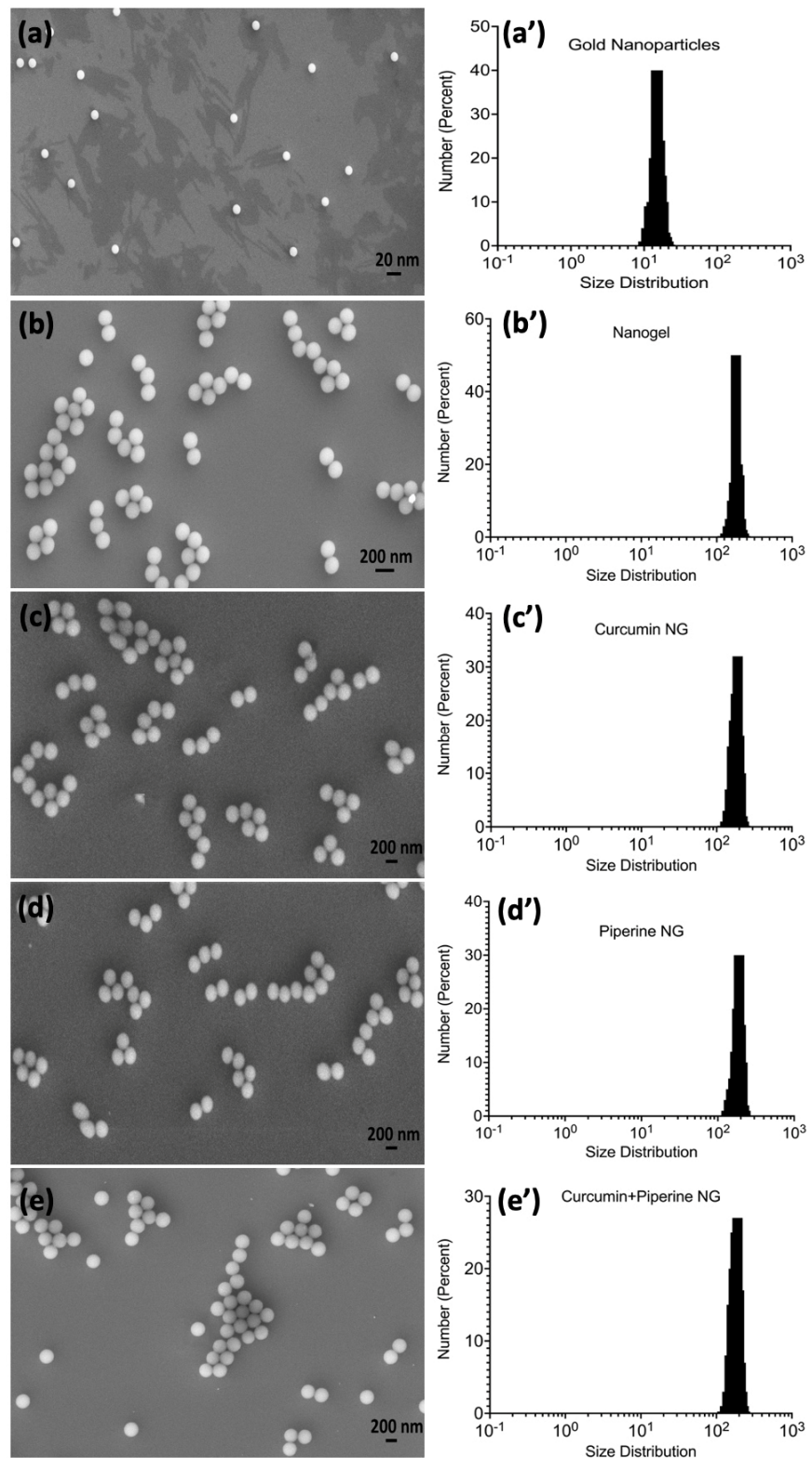
Figure 2. A scanning electron microscopic images and size distribution analysis of nano-formulations; (a) gold nanoparticles; (b) gold nanoparticles and nanogel; (c) curcumin-loaded gold nanogel; (d) piperine-loaded gold nanogel; (e) hybrid curcumin–piperine-loaded gold nanogel; (a') size distribution analysis of gold nanoparticles; (b') size distribution analysis of nanogel; (c') size distribution analysis of curcumin-loaded nanogel; (d') size distribution analysis of piperine-loaded nanogel; (e') size distribution analysis of curcumin–piperine-loaded nanogel.
