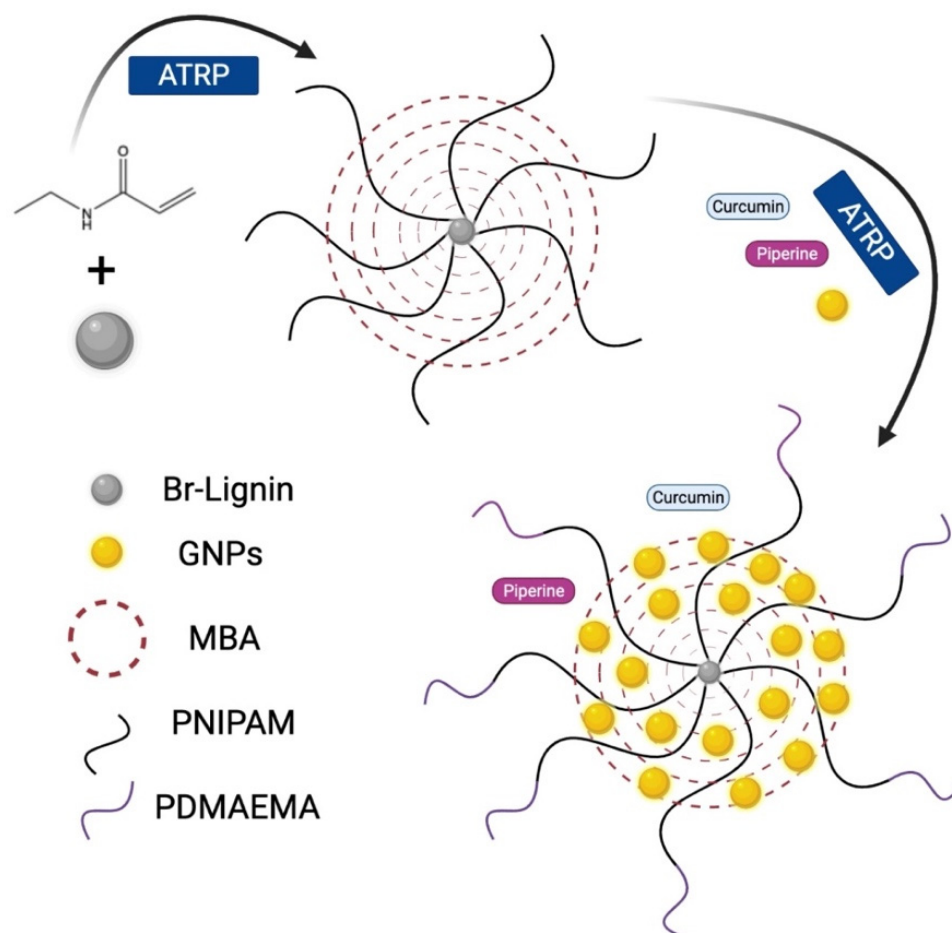
Figure 1. Schematic representation of the synthesis of Lignin-g- p (NIPAM-co-DMAEMA) gold nanogels.
