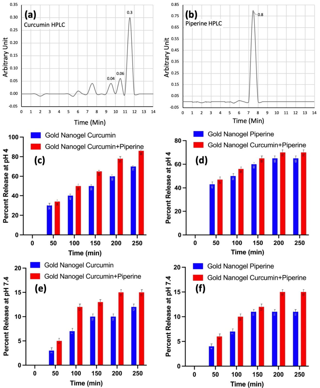
Figure 3. Determination of drug release kinetics; (a) curcumin HPLC; (b) piperine HPLC; (c) kinetic release of curcumin from nanogels at pH 4; (d) kinetic release of piperine from nanogels at pH 4; (e) kinetic release of curcumin from nanogels at pH 7.4; (f) kinetic release of piperine from nanogels at pH 7.4.
