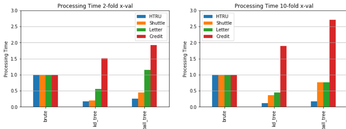
Fig. 7. Processing time for Kd-Tree and Ball Tree compared with brute force search. Times are normalised to the brute force time. ( < 1 is an improvement), 2-fold cross validation on the left and 10-fold on the right.
