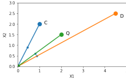
Fig. 2. Cosine Similarity: Q , C & D are three examples in a 2D feature space, using Cosine Similarity the nearest neighbour to Q is D .
