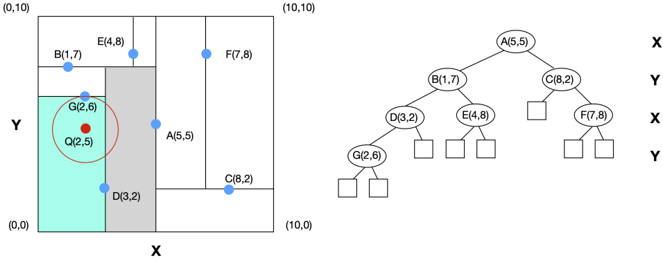
Fig. 6. A Kd-Tree based on the example in the original paper by Bentley [7]. The partitioning of the 2D feature space shown on the left corresponds to the tree on the right.
