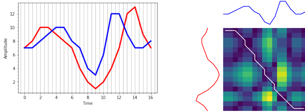
Fig. 5. The image on the left illustrates the main challenge in quantifying similarity between time-series. The two series are similar but the Euclidean distance between them is large. The image on the right shows the DTW mapping between the two time-series (produced using tslearn[51]).
