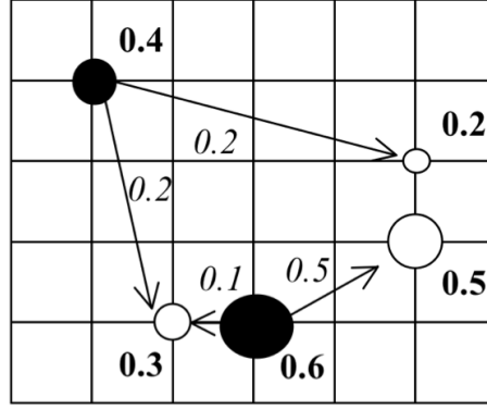
Fig. 4. An example of the EMD between two 2D signatures with two points (clusters) in one signature and three in the other (based on example in [44]).
