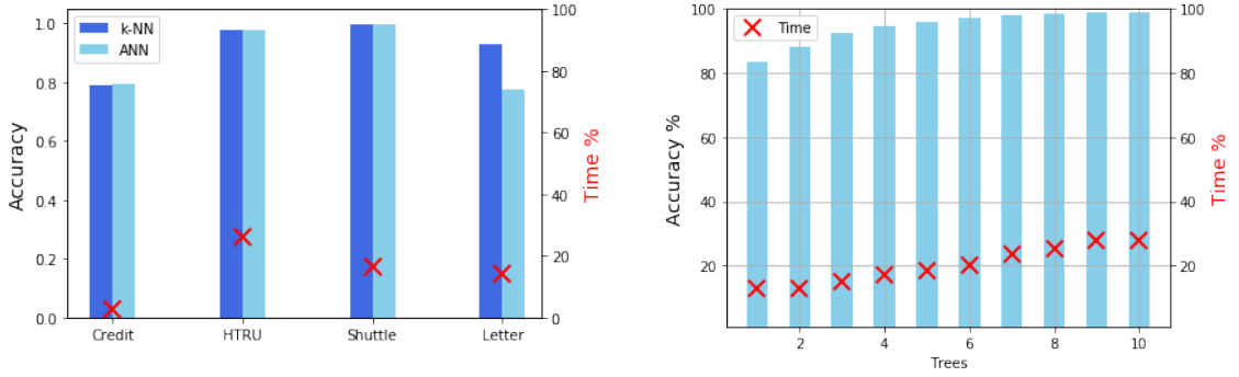
Fig. 8. The plot on the left shows the accuracy of ANN using a single tree compared with ‘full search’ k -NN. The time saving is significant. The plot on the right shows that accuracy on the Letter dataset can be improved with the addition of more trees.
