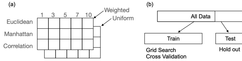
Fig. 16. (a) Grid Search for k -NN considering k , the distance metric and instance weighting policy (Weighted or Uniform). (b) Typically, Grid Search will be performed on the training data with the impact assessed on a hold-out set.
