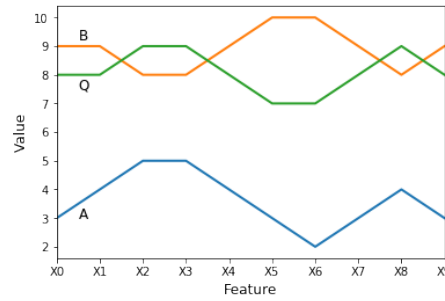
Fig. 3. Correlation: Q, A & B are three examples described by 10 features ( X_0 - X_9 ), correlation recognises that Q is more similar to A than to B.
