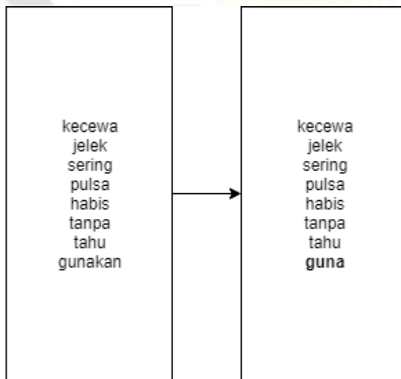
Gambar 3.8 Contoh Proses Stemming
