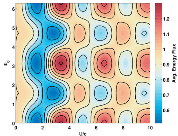
FIG. 4. Tidally averaged baroclinic energy flux ( \langle F \rangle = \langle u'p' \rangle ), where u' and p' are defined using Eq. (7) with A = 1 and with the time mean removed; \langle F \rangle is further normalized by the case where U/c = 0 . Average fluxes vary with \Phi_0 but generally reach a minimum where U/c \sim 2 and a maximum where U/c \sim 3 . Contours are spaced 0.1 units apart.
