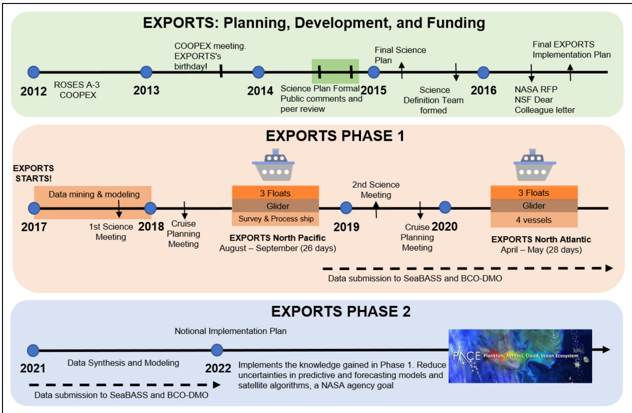
Figure 4. Timeline for the NASA EXPORTS Field Campaign. Shown here is the original NASA time line for the EXPORTS Field Campaign before postponement of the 2020 North Atlantic cruise due to the COVID-19 pandemic. The three boxes arranged vertically illustrate the planning, development and funding period (upper green), the Phase 1 field program (middle tan), and the planned Phase 2 data synthesis and modeling program (bottom blue). The NE Pacific cruise, the subject of this special collection of Elementa , is the first major field deployment for the Phase 1 program. The second field deployment to the North Atlantic was postponed due to the COVID-19 pandemic, but is underway at the time of manuscript acceptance (May 2021). The postponement of the second field deployment also pushes the start date for the Phase 2 program forward by at least a year. DOI: https://doi.org/10.1525/elementa.2020.00107.f4
