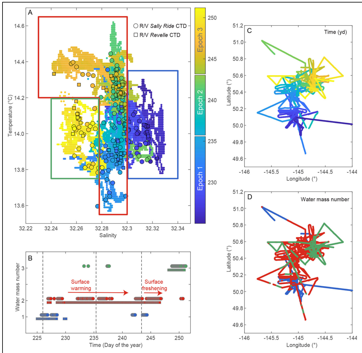
Figure 16. Variations in surface mixed layer water masses. (A) Distribution of temperature (°C) and salinity from underway measurements (both ships, dots) as well as R/V Ride (circles) and R/V Revelle (squares) CTD casts. For all symbols, color indicates the time of the measurement (year day). Three water masses, outlined by blue, red, and green curves, delineate separate water mass properties (see text for details). (B) Time series of the three surfaces water masses encountered by the R/V Ride (circles) and R/V Revelle (squares). The water mass identification is discretized in 0.2-day bins. Maps of the R/V Ride and Revelle positions colored by (C) time (year day) and (D) water mass index are shown in the right-hand panels. DOI: https://doi.org/10.1525/elementa.2020.00107.f16
