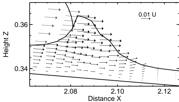
Fig. 9. Experiment B: Relatively soft and moderately non-linear till ( m = 3 , B = 0.35 ): Velocity vectors of the sediment bulge are shown at the dimensionless time T = 15 . Velocity vectors are mostly parallel to the bed. Sediment uplift takes place at the down-facing side of the bulge.
