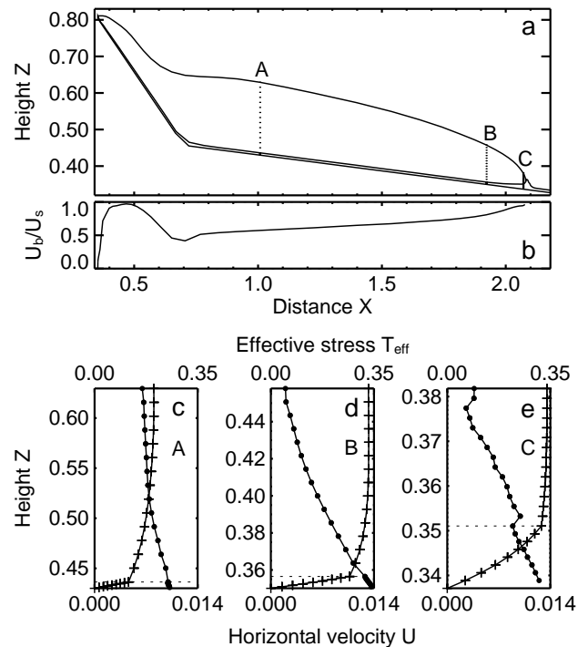
Fig. 10. Experiment B: Relatively soft and moderately non-linear till ( m = 3 , B = 0.35 ): (c–e) vertical profiles of the non-dimensional horizontal velocity U (lines with crosses) and effective stress T_{\text{eff}} (lines with dots) are shown at a dimensionless time T = 15 for the three locations A, B and C shown in (a). Note that the vertical scale changes for each profile. (b) shows the ratio between the horizontal velocity at the ice-sediment interface U_b to the one at the glacier surface U_s .
