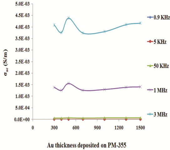
Fig. 8 — AC conductivity versus different Au thickness at frequencies 0.9 kHz, 5 kHz, 50 kHz, 1 MHz and 3 MHz.
