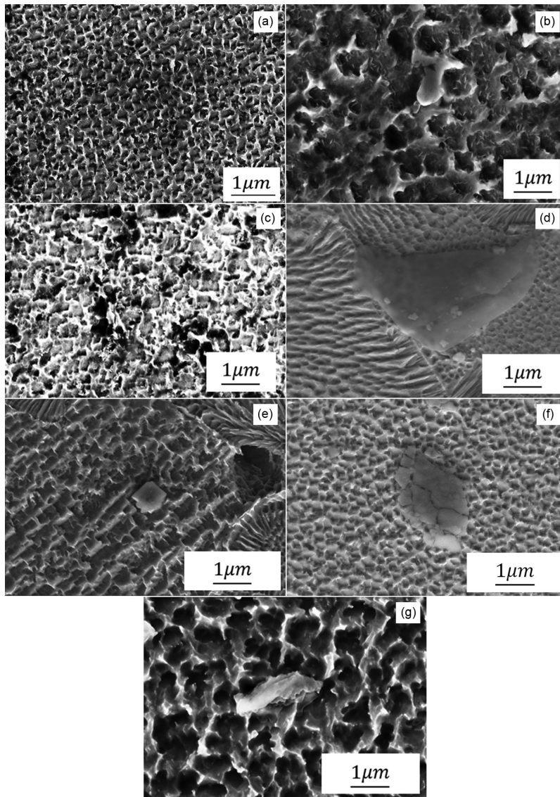
Fig. 4 — The microstructure of the Nickel-based superalloy GH4720Li under different conditions: (a) initial microstructure, (b) 10\text{s}^{-1} , 20^\circ\text{C} , (c) 10\text{s}^{-1} , 800^\circ\text{C} , (d) 1000\text{s}^{-1} , 20^\circ\text{C} , (e) 1000\text{s}^{-1} , 800^\circ\text{C} , (f) 5000\text{s}^{-1} , 20^\circ\text{C} , and (g) 5000\text{s}^{-1} , 800^\circ\text{C}
