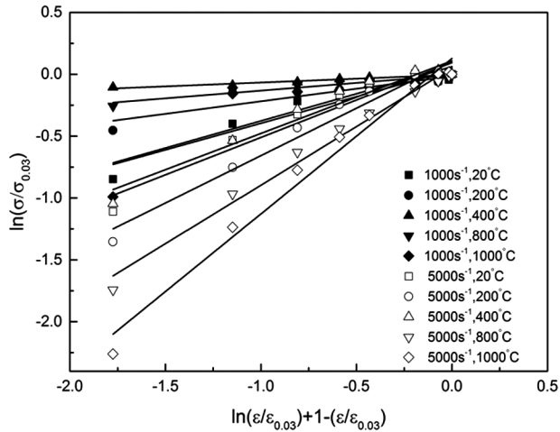
Fig. 11 — Relationship between [\ln(\frac{\epsilon}{\epsilon_{0.03}}) + (1 - \frac{\epsilon}{\epsilon_{0.03}})] - \ln(\frac{\sigma}{\sigma_{0.03}}) . \ln(\frac{\sigma}{\sigma_{0.03}}) = C[\ln(\frac{\epsilon}{\epsilon_{0.03}}) + (1 - \frac{\epsilon}{\epsilon_{0.03}})] \dots (15)
