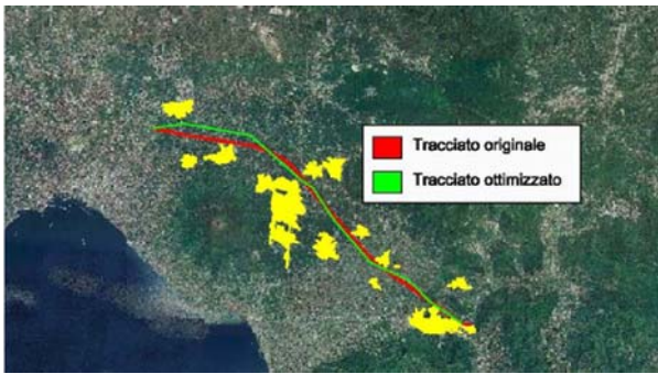
Fig. 6. Path of the high speed stretch between Salerno and Naples. In yellow the constraints in the presence of settlements
