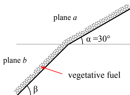
Figure 1. Double-slope plane configuration.
