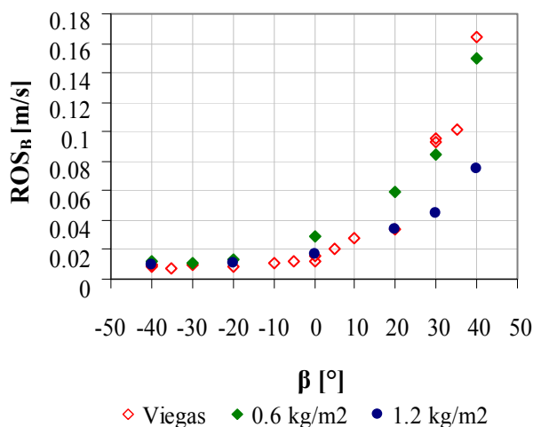
Figure 3. Comparison between the experimental and simulated rate of spread for flames moving on plane b
