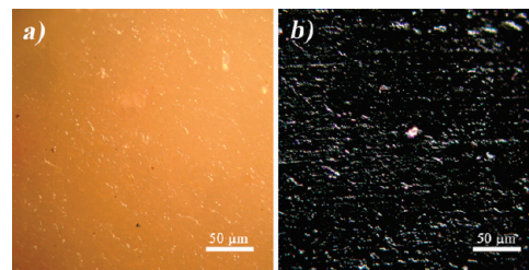
Figure 4. OM image of tensile test specimen of sample 2 (15 wt % in styrene) cut in liquid nitrogen (a) and after staining with OsO 4 (b).
