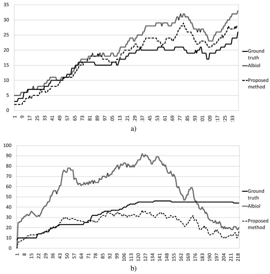
Figure 3. Curves of the number of people estimated by the Albiol's and our algorithms in each frame together with the ground truth on the video sequence S1.L1.13-59 view 1 (a) and S1.L1.13-57 view 2 (b). On the x-axis it is reported the frame number.
