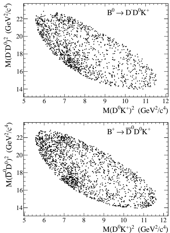
FIG. 2. Distributions of the data for the Dalitz plot for B^0 \rightarrow D^- D^0 K^+ (top) and B^+ \rightarrow \bar{D}^0 D^0 K^+ (bottom), where each dot represents a B candidate.
