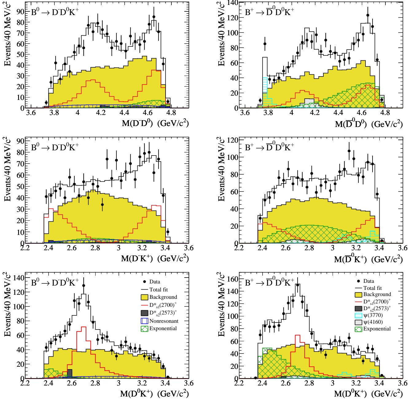
FIG. 4. Projections of the Dalitz plot on the three axes for the data (dots) and for the result of the nominal fit (total histogram) for the modes B^0 \rightarrow D^- D^0 K^+ (left) and B^+ \rightarrow \bar{D}^0 D^0 K^+ (right). The fit includes the background (plain yellow histogram), the nonresonant (vertical-hatched blue histogram, present only for B^0 \rightarrow D^- D^0 K^+ ), the D_{s1}^*(2700)^+ (red histogram), the D_{s2}^*(2573)^+ (plain dark gray histogram), and the exponential (cross-hatched green histogram) amplitudes. For B^+ \rightarrow \bar{D}^0 D^0 K^+ , the additional charmonium contributions consist of the \psi(3770) (horizontal-hatched light blue histogram) and the \psi(4160) (plain light gray histogram) amplitudes.
