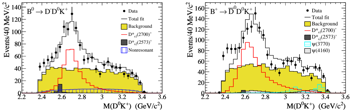
FIG. 3. Projections of the Dalitz plot on the D^0 K^+ axis for the data (dots) and for the result of the preliminary fit (total histogram) for the modes B^0 \rightarrow D^- D^0 K^+ (left) and B^+ \rightarrow \bar{D}^0 D^0 K^+ (right). The fit includes the background (plain yellow histogram), the nonresonant (vertical-hatched blue histogram), the D_{s1}^*(2700)^+ (red histogram), and the D_{s2}^*(2573)^+ (plain dark gray histogram) amplitudes. For B^+ \rightarrow \bar{D}^0 D^0 K^+ , the additional charmonium contributions consist of the \psi(3770) (horizontal-hatched light blue histogram) and the \psi(4160) (plain light gray histogram) amplitudes.
