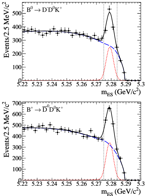
FIG. 1. Fits of the m_{ES} data distributions [15] for the modes B^0 \rightarrow D^- D^0 K^+ (top) and B^+ \rightarrow \bar{D}^0 D^0 K^+ (bottom). Points with statistical errors are data events, the red dashed line represents the signal PDF, the blue dashed line represents the background PDF, and the black solid line shows the total PDF. The vertical lines indicate the signal region used in the rest of the analysis.
