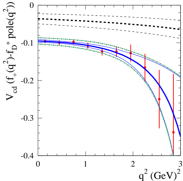
FIG. 10: Contributions of high-mass poles to |V_{cd}| \times f_{+,D}^\pi(q^2) . For all data and projections the D^{*+} contributions are subtracted: data points (red) represent the measurements (Fig. 8) and the full (blue) curve, with thin lines on both sides, represents the fit result and uncertainties in the z -expansion parameterization, the dash-dotted lines indicate the additional uncertainties from the pole estimate. The dashed black lines mark the expected contribution from the D_1^{*+} pole (see Eq. (A3)) and corresponding uncertainties.
