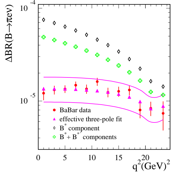
FIG. 12: Comparison of the measured differential branching fraction for B^0 \rightarrow \pi^- e^+ \nu_e [46], integrated over 2 \text{ GeV}^2 q^2 intervals (apart from the last bin which extends from 22 to 26.2 \text{ GeV}^2 ), with expectations from the effective three-pole ansatz. The two lines indicate theoretical uncertainties on these predictions. The contributions from the B^* pole and from the sum of the B^* and B_1' poles are indicated.
