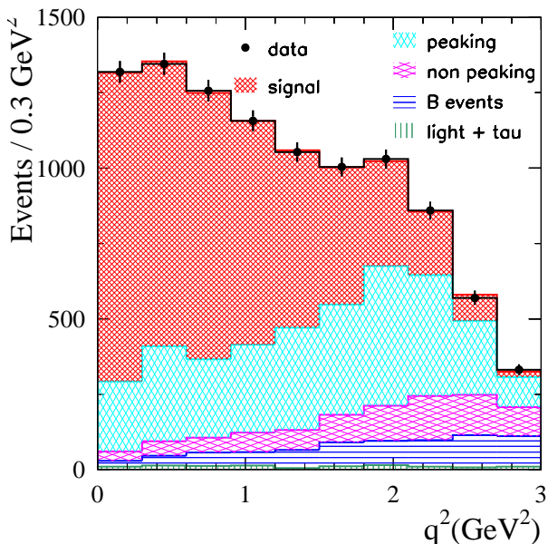
FIG. 3: The measured q^2 distribution (data points) for events selected in the \Delta(m) signal region is compared to the sum of the estimated backgrounds and the fitted signal components. Peaking and non-peaking background contributions refer only to c\bar{c} events.
