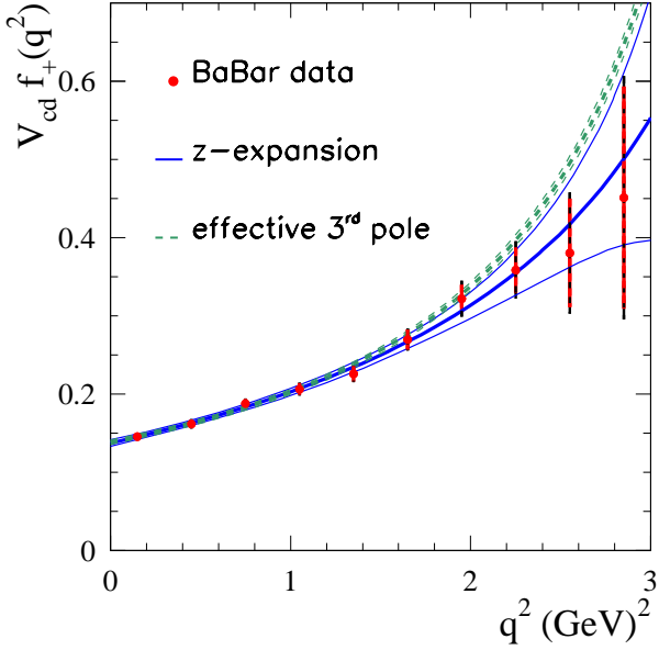
FIG. 8: Measured values of |V_{cd}| \times f_{+,D}^\pi(q^2) are compared with the results of a fit using a z -expansion parameterization of the hadronic form factor (full blue line). The dashed (green) lines show the comparison with a fit using the effective three-pole ansatz in which the mass of an effective third pole is fitted. The superconvergence condition and constraints on the two first residues are imposed (see Section VI C 4).
