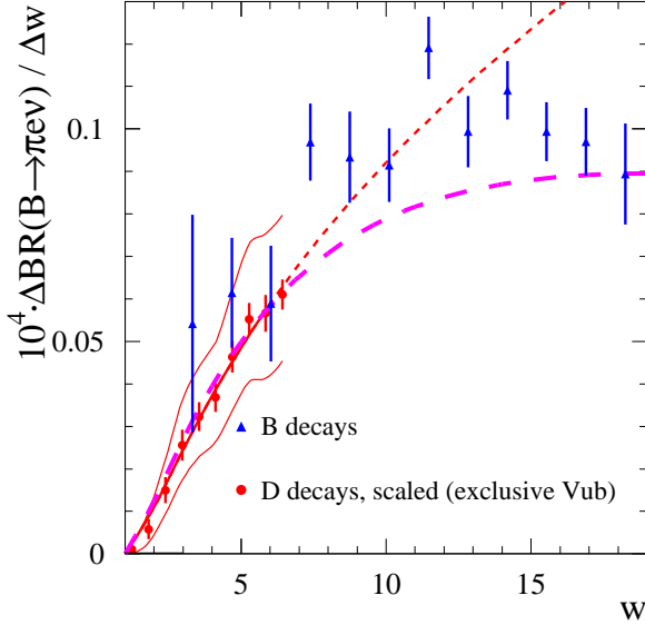
FIG. 11: Comparison of the dB^B/dw differential decay rate for B^0 \rightarrow \pi^- e^+ \nu_e decays measured by BABAR with an extrapolation of the D^0 \rightarrow \pi^- e^+ \nu_e form factor measurement. The solid red line is the result of the fit to the fixed three-pole ansatz with m_{\text{pole}3} = 3.1 \text{ GeV}/c^2 , the short-dash red line marks the extrapolation beyond the physical region for the D^0 \rightarrow \pi^- e^+ \nu_e decay. The two thin red lines indicate the impact of the 12% uncertainty on the form factor ratio R_{BD} . The long-dash magenta line marks the fit result, to D^0 \rightarrow \pi^- e^+ \nu_e data, for the effective three-pole ansatz. In these comparisons, the value |V_{ub}|^{\text{excl.}} is used.
