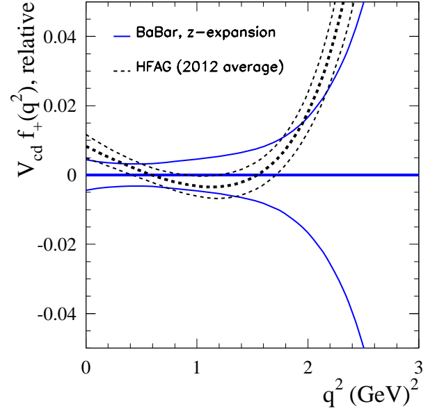
FIG. 9: Comparison of this measurement with an average by HFAG of all other results listed in Table VII, both obtained from fits to the z -expansion. For the curves and their error bands the BABAR results in Fig. 8 have been subtracted. The continuous (blue) lines illustrate total uncertainties in the BABAR measurement, for which the central values are, by construction, equal to zero. Dashed (black) lines are the results of HFAG.
