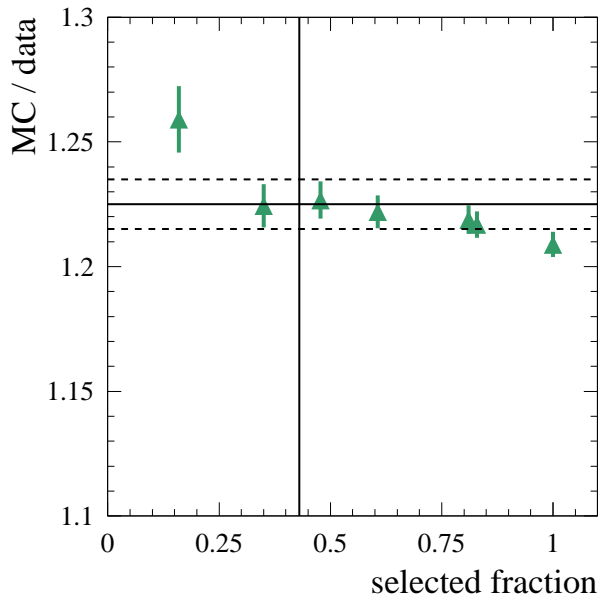
FIG. 6: Variation of the ratio of numbers of D^0 \rightarrow K^- \pi^+ events measured in MC and data, as a fraction of events selected by restrictions on F_{c\bar{c}-2} . The vertical line shows the fraction of selected D^0 \rightarrow \pi^- e^+ \nu_e events after the requirement on F_{c\bar{c}} . All events satisfy F_{b\bar{b}} > 1.2 . The horizontal lines indicate the value adopted for this ratio (full line) and the corresponding uncertainty (dashed lines).
