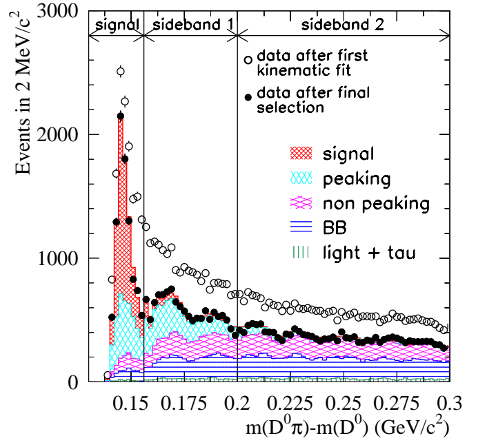
FIG. 2: Mass difference \Delta(m) = m(D^0\pi_s^+) - m(D^0) after all selection criteria and the additional requirement on the first (open circles) and second (full circles) kinematic fits probabilities. The distribution for MC-simulated signal and the different background distributions are superimposed for the final selections. These MC distributions are normalized to data based on the integrated luminosity and have been corrected to account for small differences between data and MC distributions.
