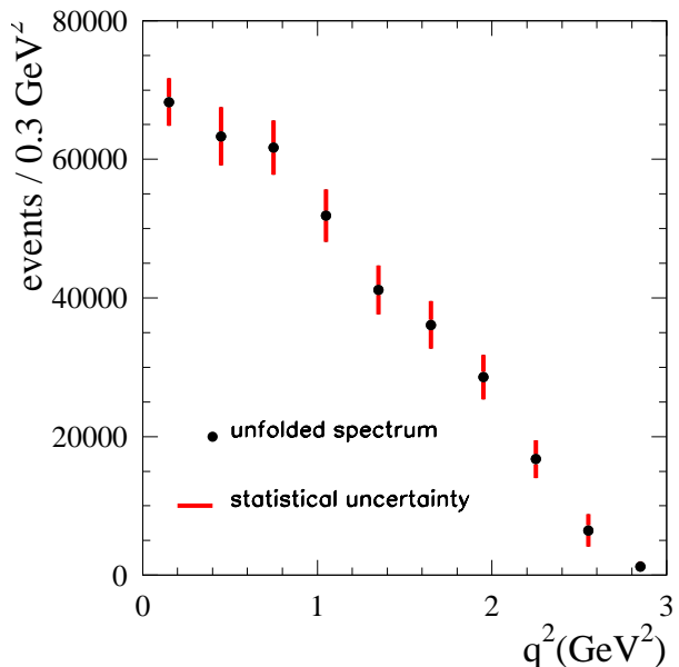
FIG. 7: Unfolded q^2 distribution for D^0 \rightarrow e^+ \pi^- \nu_e decays.
