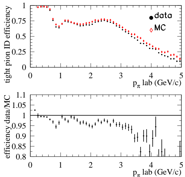
FIG. 4: Study of the uncorrected pion efficiency in data and in simulation versus the laboratory pion momentum; top: measured efficiencies, bottom: ratio of efficiencies in data and MC.
