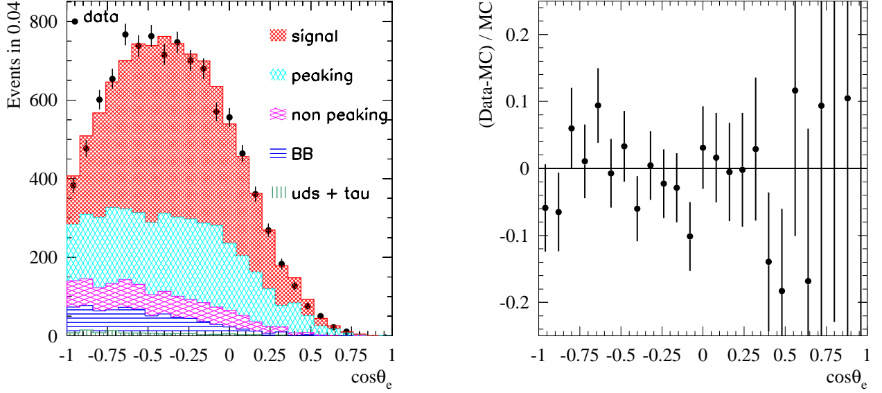
FIG. 5: Comparison of the measured event yields (black data points with statistical errors), as a function of \cos\theta_e , with the corrected sum of the expected signal and background distributions after all corrections. Left: observed events in data and in simulation. Right: the ratio (\text{Data} - \text{MC})/\text{MC} .
