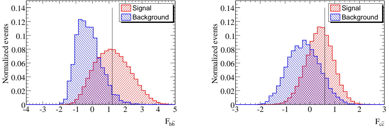
FIG. 1: Distributions of the Fisher discriminants; Left: F_{b\bar{b}} for signal and B\bar{B} events, Right: F_{c\bar{c}} for signal and other c\bar{c} events. The vertical lines indicate the selection requirements: F_{b\bar{b}} > 1.2 and F_{c\bar{c}} > 0.6 .
