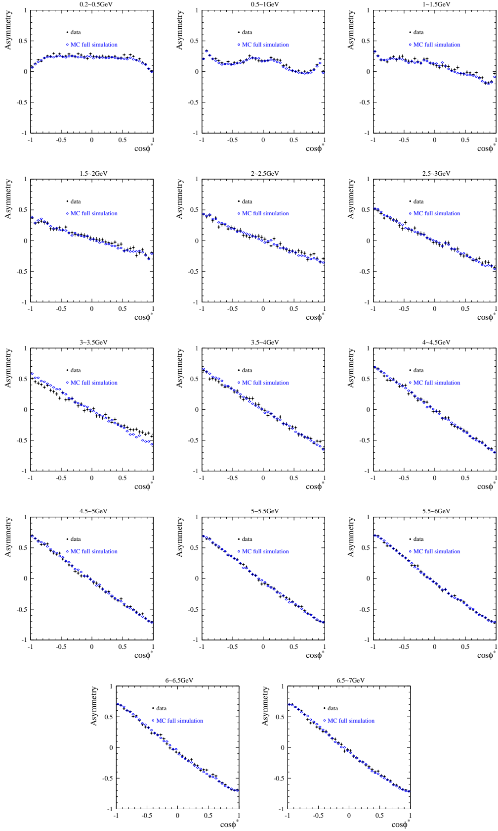
FIG. 14: Raw charge asymmetry as a function of \cos \phi^* for \mu^+ \mu^- \gamma events in data ( \bullet ) and MC ( \circ ), in various m_{\mu\mu} intervals, after the complete event selection.
