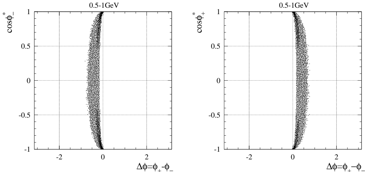
FIG. 13: (left) Distribution of \cos \phi^* vs. \Delta\phi for the N_- sample ( \phi^* \in [0, \pi] ) in the (0.5–1.0) \text{GeV}/c^2 mass interval for the \mu^+\mu^-\gamma MC; (right) the same for the N_+ sample ( \phi^* \in [0, \pi] )
