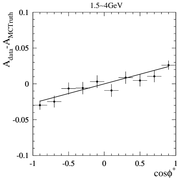
FIG. 20: The difference between the measured asymmetry in the \mu^+\mu^-\gamma process and the QED prediction, as implemented in AfkQed, as a function of \cos\phi^* for the events in the mass interval 1.5\text{--}4\text{ GeV}/c^2 , excluding the J/\psi 3.0\text{--}3.2\text{ GeV}/c^2 region. The result of a linear fit is shown by the solid line.
