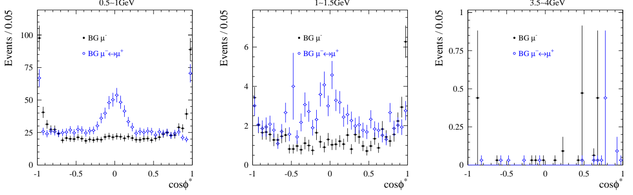
FIG. 8: Backgrounds estimated with MC for e^+e^- \rightarrow \mu^+\mu^-\gamma as a function of \cos\phi^* in selected m_{\mu\mu} intervals. The points labeled ' \mu^- ' refer to the configurations with \phi_-^* \in [0, \pi] , while the points labeled ' \mu^- \leftrightarrow \mu^+ ' correspond to \phi_+^* \in [0, \pi] .
