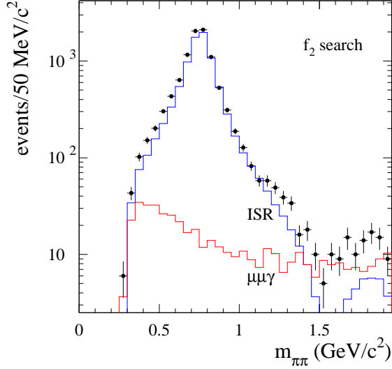
FIG. 26: The \pi\pi mass spectrum for |\cos\theta^*| > 0.85 for the analysis extended to low momentum (points), the expected background from misidentified \mu\mu\gamma events (red histogram), and the predicted ISR spectrum from the standard cross section analysis (blue histogram).
