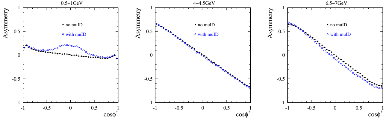
FIG. 12: Raw charge asymmetry as a function of \cos\phi^* in selected m_{\mu\mu} intervals, for e^+e^- \rightarrow \mu^+\mu^-\gamma MC events with ( \circ ) and without ( \bullet ) the two-muon identification, where the events are already required to be within the kinematic acceptance and have two good charged-particle tracks reconstructed.
