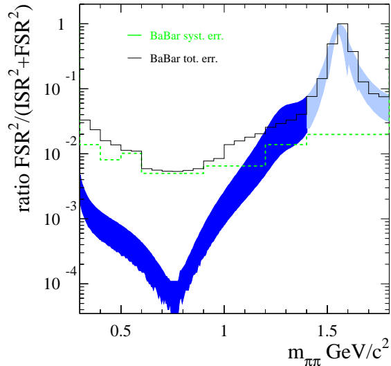
FIG. 29: The FSR fraction in the BABAR measurement [6] of the \pi\pi\gamma cross section, defined as the ratio \frac{|\mathcal{M}_{\text{FSR}}|^2}{|\mathcal{M}_{\text{ISR}}|^2 + |\mathcal{M}_{\text{FSR}}|^2} obtained in this analysis using FSR model 2 with c_{0,2} parameters fitted to data (blue band). The light-blue part corresponds to the extrapolation of the model beyond the fitted range. The FSR fraction is compared to the systematic error of the BABAR cross section measurement (green dashed histogram) and its total error (black histogram).
