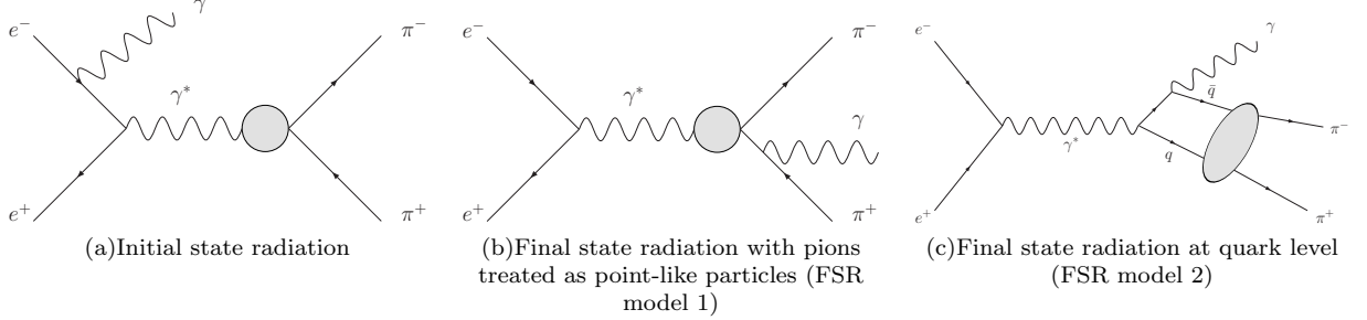
FIG. 5: Feynman diagrams for e^+e^- \rightarrow \pi^+\pi^-\gamma .
