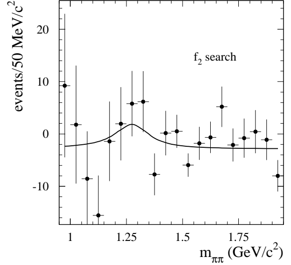
FIG. 27: The \pi\pi mass spectrum for |\cos\theta^*| > 0.85 for the analysis extended to low momentum (points) after subtraction of the \mu\mu\gamma background and the ISR contribution. The curve is the result of a fit to a constant term and a simple Breit-Wigner shape for the f_2 resonance.
