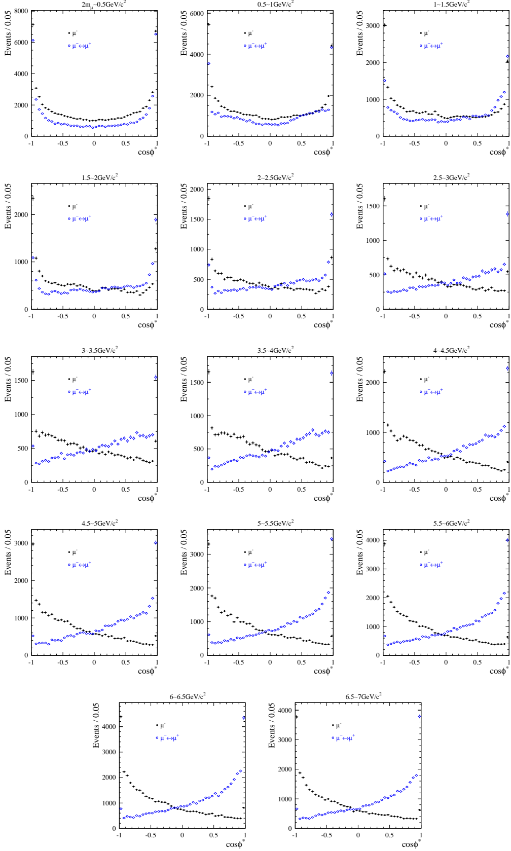
FIG. 6: The \cos\phi^* distributions for e^+e^- \rightarrow \mu^+\mu^-\gamma data in 0.5\text{ GeV}/c^2 m_{\mu\mu} intervals. The points labeled ' \mu^- ' refer to the configurations with \phi_-^* \in [0, \pi] , while the points labeled ' \mu^- \leftrightarrow \mu^+ ' correspond to \phi_+^* \in [0, \pi] .
