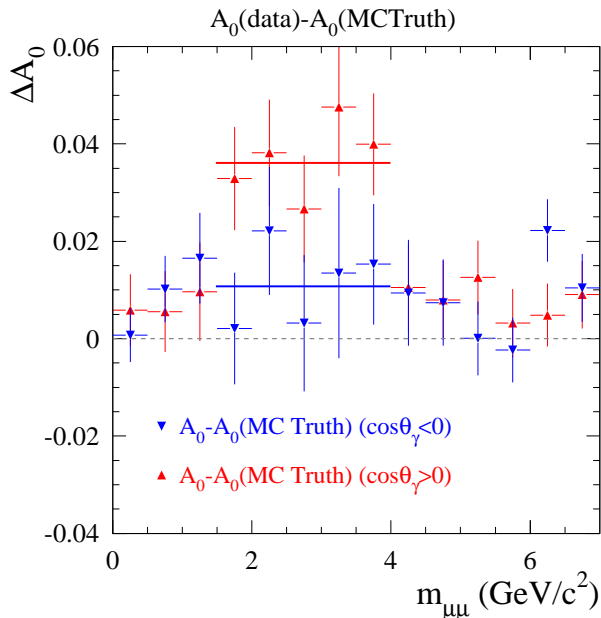
FIG. 18: The difference between the measured asymmetry slope in the \mu^+\mu^-\gamma process and the AfkQed prediction, as a function of m_{\mu\mu} , excluding the J/\psi 3.0-3.2 GeV/ c^2 region. Forward ( \cos\theta_\gamma^* > 0 ) and backward ( \cos\theta_\gamma^* < 0 ) hemispheres are analysed separately. Statistical uncertainties only.
