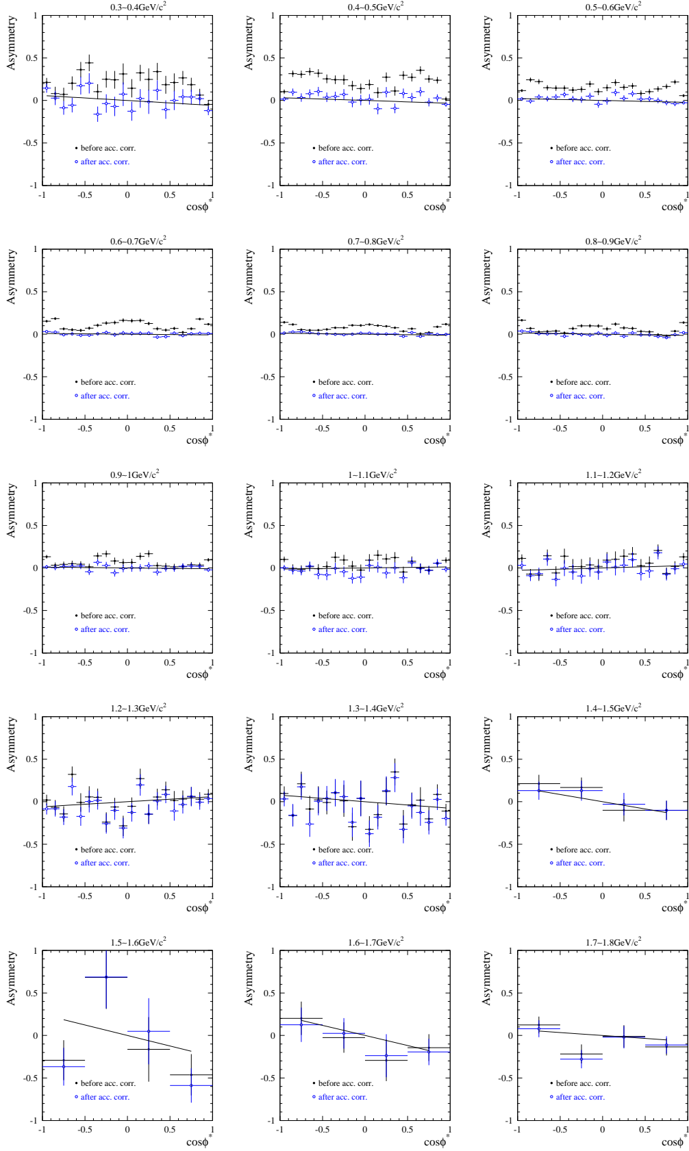
FIG. 21: Charge asymmetry for e^+e^- \rightarrow \pi^+\pi^-\gamma data before ( \bullet ) and after ( \circ ) efficiency corrections, in 0.1 \text{GeV}/c^2 mass intervals from 0.3 \text{GeV}/c^2 to 1.8 \text{GeV}/c^2 . The line shows the result of the fit to A_0 \cos\phi^* .
