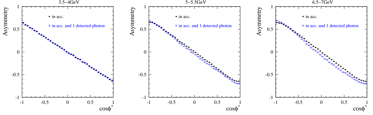
FIG. 11: Raw charge asymmetry as a function of \cos\phi^* in selected m_{\mu\mu} intervals, for e^+e^- \rightarrow \mu^+\mu^-\gamma MC events with ( \circ ) and without ( \bullet ) the requirement of the reconstruction of the ‘ISR’ photon, where the events are already required to be within the kinematic acceptance.
