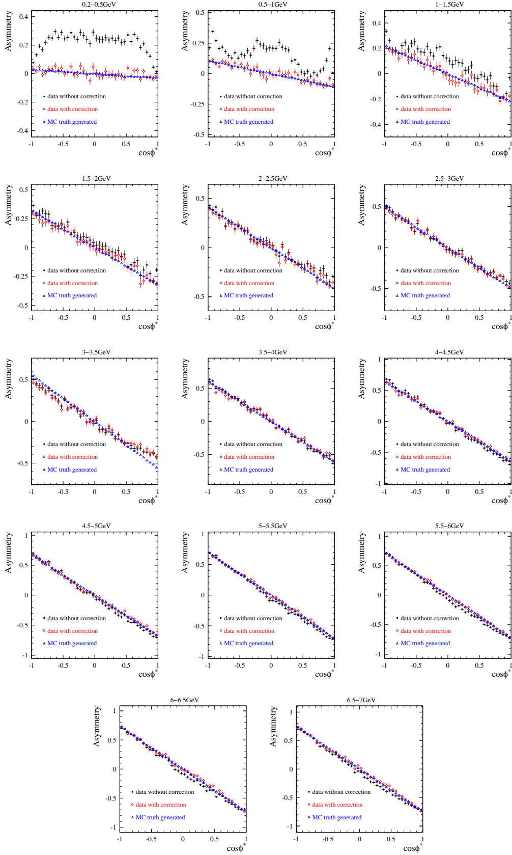
FIG. 15: Charge asymmetry in e^+e^- \rightarrow \mu^+\mu^-\gamma data before ( \bullet ) and after ( \circ ) background subtraction and efficiency corrections, and for MC ( \triangle ) at generation level.
