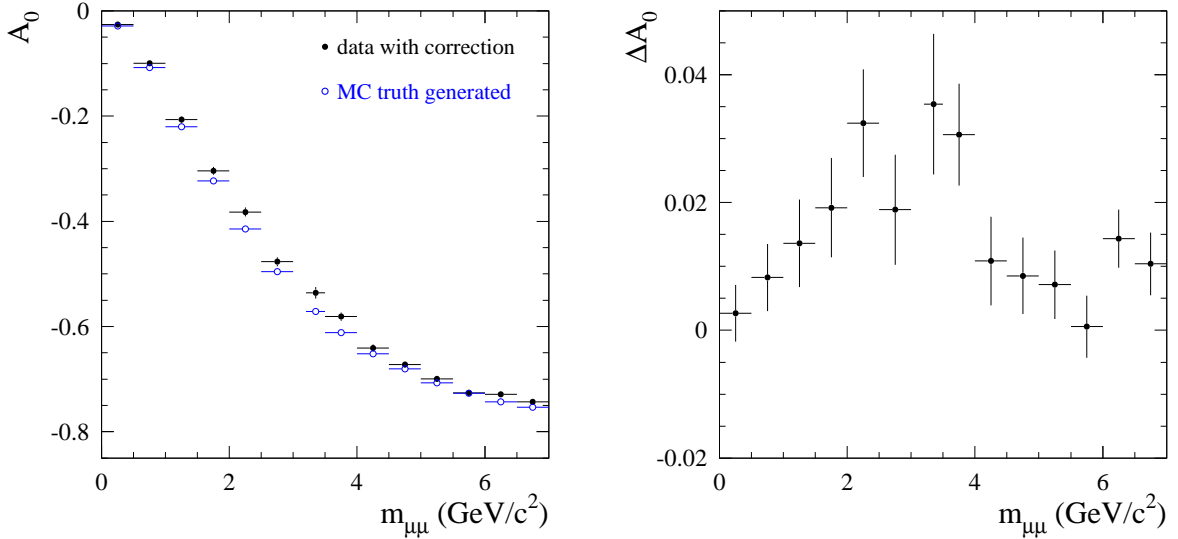
FIG. 17: The slope A_0 of charge asymmetry as a function of m_{\mu\mu} in e^+e^- \rightarrow \mu^+\mu^-\gamma data and in MC at generation level (left), and the absolute difference between them (right). The J/\psi mass region ( 3.0\text{-}3.2\text{ GeV}/c^2 ) is excluded. Only statistical uncertainties are shown.
