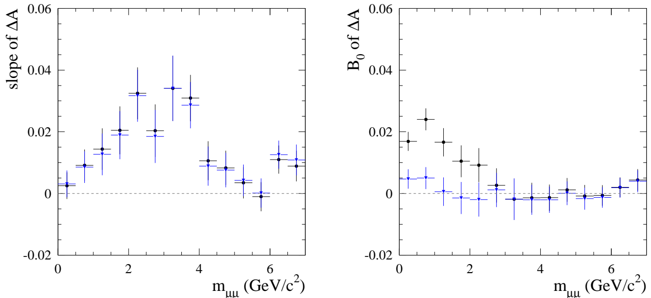
FIG. 19: (left) Slope of the difference \Delta A^{\text{raw}}(\cos \phi^*) for \mu^+\mu^-\gamma between the raw asymmetries observed in data and in MC before (black points) and after (blue triangles) the data/MC corrections, as a function of m_{\mu\mu} . (right) Constant term of the two-parameter linear fits of \Delta A^{\text{raw}}(\cos \phi^*) . Statistical uncertainties only.
