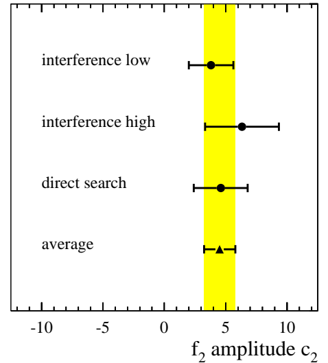
FIG. 28: The results obtained for the f_2(1270) amplitude c_2 in the process e^+e^- \rightarrow \pi^+\pi^-\gamma from the interference analysis and the direct f_2(1270) search in the cross section. The labels ‘low’ and ‘high’ refer to the determination in the two angular ranges |\cos\theta^*| < 1/\sqrt{3} and 1/\sqrt{3} < |\cos\theta^*| . For the direct search the positive solution is chosen. The combined value for the three independent analyses is given by the vertical band.
