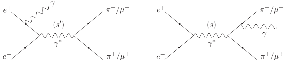
FIG. 1: Feynman diagrams for e^+e^- \rightarrow x^+x^-\gamma ( x = \mu, \pi ), where the photon is from lowest order initial state radiation (LO ISR, left) or lowest order final state radiation (LO FSR, right).
