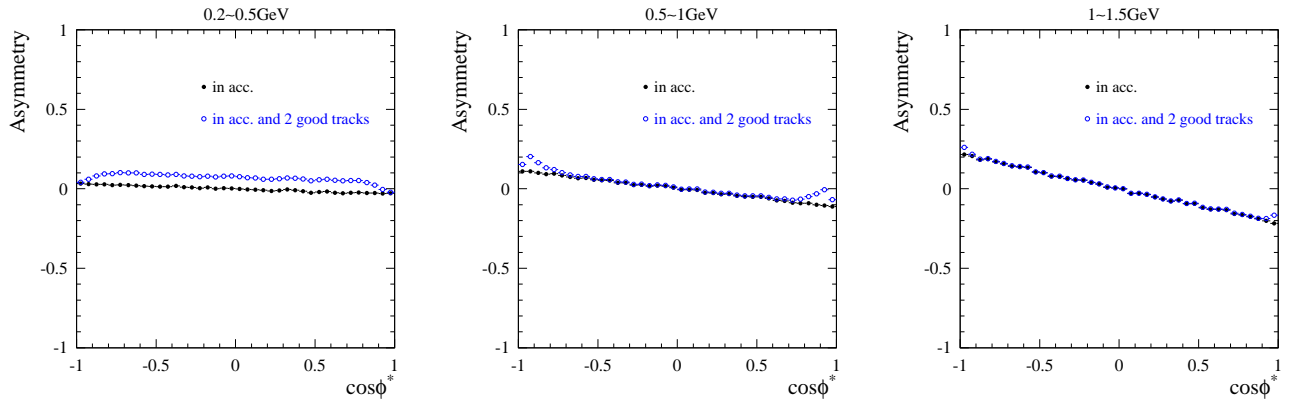
FIG. 10: Raw charge asymmetry as a function of \cos\phi^* in selected m_{\mu\mu} intervals, for e^+e^- \rightarrow \mu^+\mu^-\gamma MC events with ( \circ ) and without ( \bullet ) reconstruction of two good charged-particle tracks, where the events are already required to be within the kinematic acceptance.
