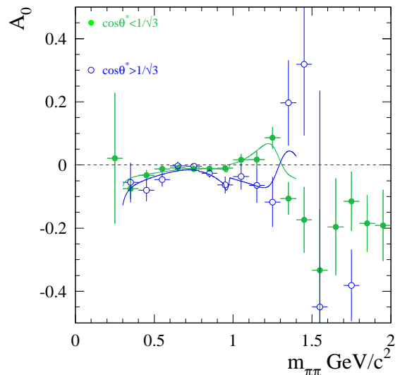
FIG. 23: The charge asymmetries measured with |\cos\theta^*| below and above 1/\sqrt{3} . The curves represent the fit results (see text).
