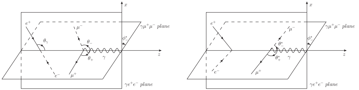
FIG. 2: Definition of the angular variables describing the kinematic topology of the final states of the process e^+e^- \rightarrow x^+x^-\gamma ( x = \mu, \pi ) at a given x^+x^- invariant mass: (left) in the e^+e^- c.m.s., (right) in the x^+x^- c.m.s.
