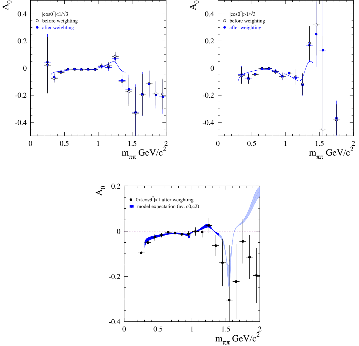
FIG. 24: The charge asymmetry slopes for e^+e^- \rightarrow \pi^+\pi^-\gamma using MC samples with and without reweighting, and fit to the model after reweighting (see text); (top left) for |\cos\theta^*| < 1/\sqrt{3} ; (top right) for |\cos\theta^*| > 1/\sqrt{3} ; (bottom) for the full |\cos\theta^*| range; the blue band represents the model-2 prediction using the average c_{0,2} values after reweighting. The light-blue part corresponds to the extrapolation of the model beyond the fitted range.
