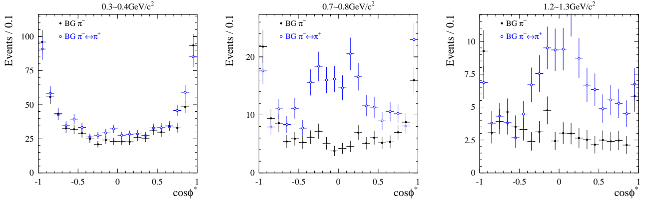
FIG. 9: Backgrounds estimated with MC for e^+e^- \rightarrow \pi^+\pi^-\gamma as a function of \cos\phi^* in selected m_{\pi\pi} intervals. The points labeled ' \pi^- ' refer to the configurations with \phi_-^* \in [0, \pi] , while the points labeled ' \pi^- \leftrightarrow \pi^+ ' correspond to \phi_+^* \in [0, \pi] .
