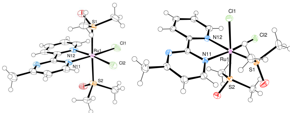
Figure 6. The X-ray structures (50% probability ellipsoids) of cis,trans -[RuCl 2 (dmsO-S) 2 (mpp- \kappa N^p )] ( 7 , left) and cis,cis -[RuCl 2 (dmsO-S) 2 (mpp- \kappa N^p )] ( 8 , right).
