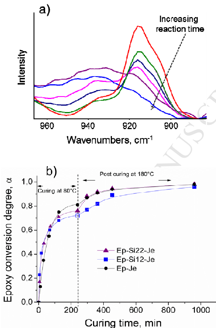
Figure 1. a) FTIR spectra of the pristine epoxy resin during the curing cycle in the region 880-965 cm -1 ; b) Conversion degree \alpha of the epoxide groups for pristine epoxy resin, Ep-Je, and the hybrid materials EP-Si12-Je and Ep-Si22-Je.
