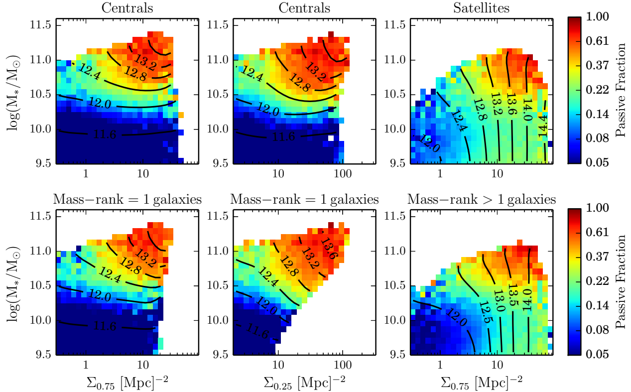
Figure 9. Fraction of passive galaxies as a function of density on the scale \Sigma_{0.75} and stellar mass for central galaxies (left panels), on the scale \Sigma_{0.25} for centrals (central panels) and on the scale \Sigma_{0.75} for satellite galaxies (right panels), at z = 1.08 . The central/satellite definition is the one provided by the SAMs in the top panels and the one defined by the mass rank in the adaptive aperture in the bottom panels. The contours are drawn from the median halo mass in the same bins.
