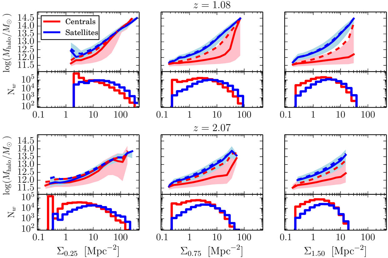
Figure 2. Median mass of the parent halo of each galaxy as a function of density measured on three scales \Sigma_{0.25} (left panels), \Sigma_{0.75} (central panels), and \Sigma_{1.50} (right panels) for central galaxies (red solid lines) and satellites (blue solid lines) at z = 1.08 (top panels), and z = 2.07 (bottom panels). The shaded areas are bounded by the 25th and 75th percentiles of the distributions. Dashed lines correspond to the mass of the most massive halo within 1 Mpc ( M_{h,1\text{Mpc}} , see text). The distribution of densities for centrals and satellites are shown in the lower part of each panel.
