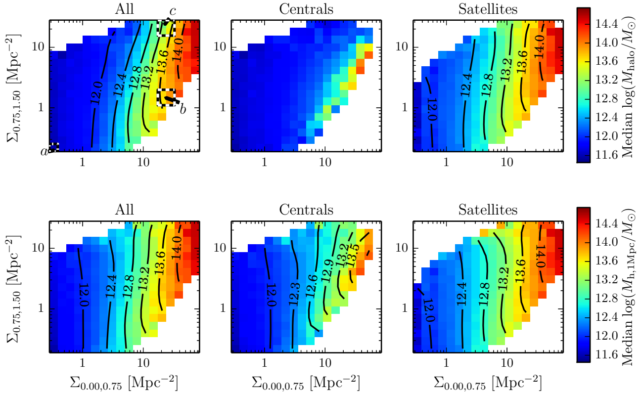
Figure A1. Top panels: halo mass dependence with density on scales \Sigma_{0.00,0.75} and \Sigma_{0.75,1.50} for all galaxies (left panels), central galaxies only (central panels) and satellite galaxies only (right panels) at z = 1.08 . Bottom panels: as before but the nominal halo mass has been replaced with that of the most massive halo within a 3D physical sphere of 1Mpc radius ( M_{h,1Mpc} ). The labels a , b , and c in the top left panel highlight three bins (black and white squares) whose halo mass distributions are shown in Figure A2.
