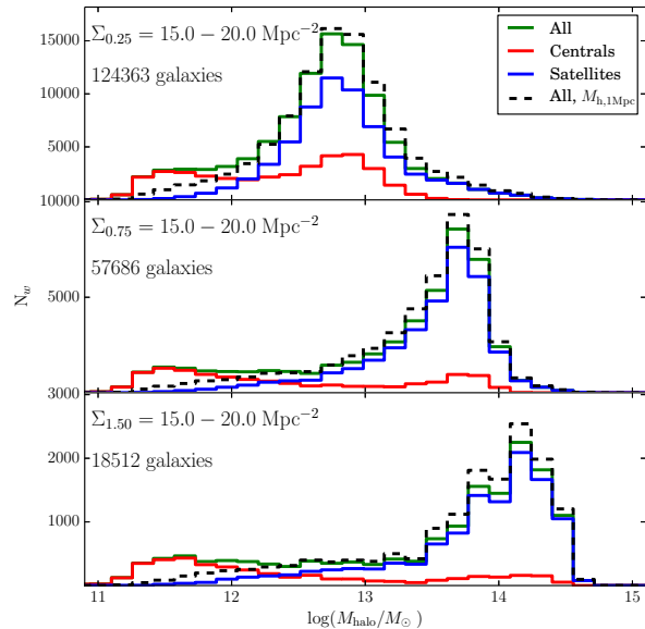
Figure 3. Weighted distributions of parent halo mass for each galaxy in a fixed bin of density ( 15\text{--}20 \text{Mpc}^{-2} ) on scales \Sigma_{0.25} (top panel), \Sigma_{0.75} (middle panel), and \Sigma_{1.50} (bottom panel) at z = 1.08 . The dashed line shows the weighted distribution of the most massive halo mass within 1 Mpc of each galaxy (see text).
