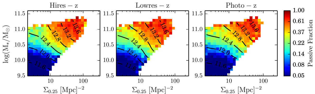
Figure 10. Fraction of passive galaxies as a function of density on the scale \Sigma_{0.25} and stellar mass for mass rank 1 galaxies (in the adaptive aperture) using hires- z (left panel), lowres- z (central panel), and photo- z (right panel) at z = 1.08 . The contours are drawn from the median halo mass in the same bins.
