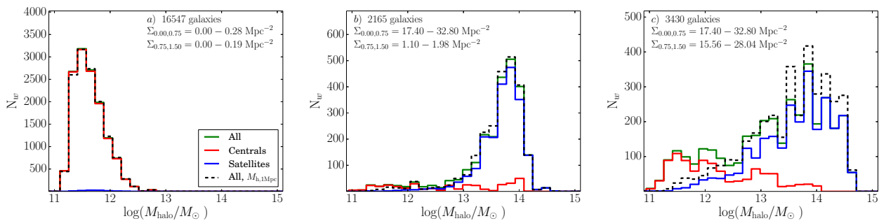
Figure A2. Halo mass distribution in three bins indicated using black and white squares and labelled a , b , and c in the top left panel of Figure A1.
