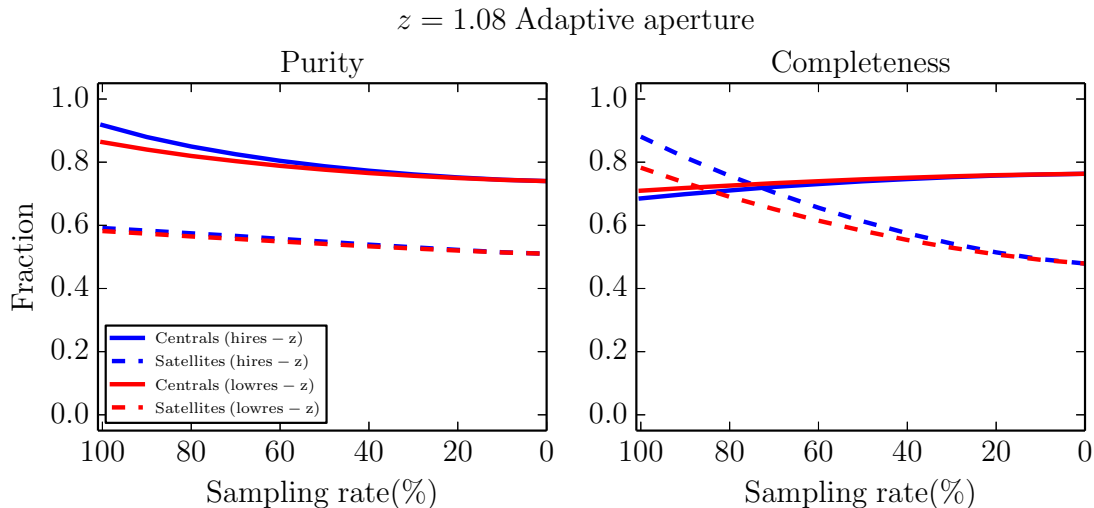
Figure 7. Purity and completeness for the identification of central (solid lines) and satellite (dashed lines) galaxies using stellar mass rank = 1 ( > 1 ) in the adaptive aperture for incomplete hires-z (blue lines) and lowres-z (red lines) sampling at z = 1.08 .
