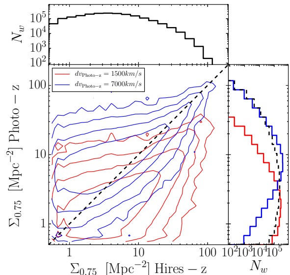
Figure 4. Main panel: Density on the 0.75 Mpc scale for the photo-z sample and different velocity cuts ( dv = 1500 \text{km/s} red and dv = 7000 \text{km/s} blue) as a function of density in the same aperture (and dv = 1500 \text{km/s} for the hires-z sample). The contours are logarithmically spaced with the outermost contours at 25 objects per bin and the innermost at 10^4 objects per bin. Upper panel: weighted distribution of density for the hires-z sample. Right panel: weighted distributions of density for the photo-z sample with the same velocity cuts as above. The distribution of density for the hires-z sample (dashed black) is repeated here for comparison.
