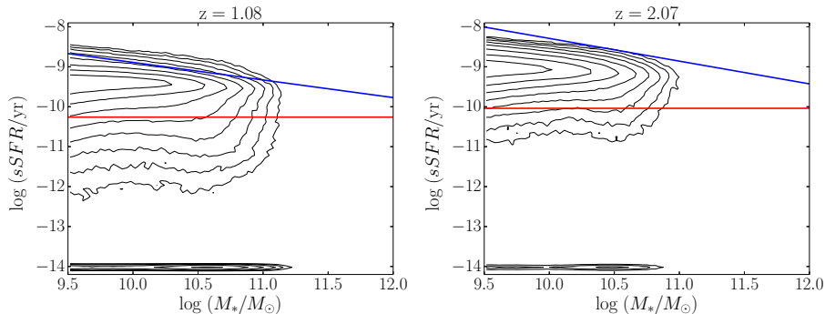
Figure 1. Specific star formation rate ( sSFR ) as a function of M_* at redshifts of 1.08 (left panel) and 2.07 (right panel). The blue line is the main sequence fit from observational data (NMBS, Whitaker et al. 2012). The red line marks the limit we set to define the passive galaxies in the models. The contour levels are log-spaced with the outermost contour at 25 objects and the innermost at 10^4 per bin. We set all galaxies with \log sSFR < -14 equal to that value.
