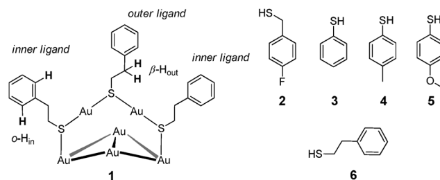
Fig. 1 Structure of the dimeric staple motif with indication of the protons monitored in the kinetic analysis of the place exchange reaction and structure of the incoming and exiting thiols used in this study.
