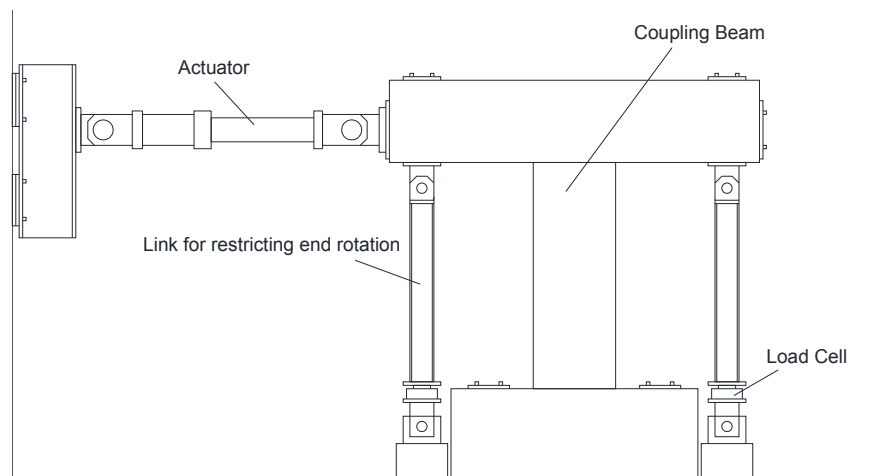
Figure 1. Test setup.
