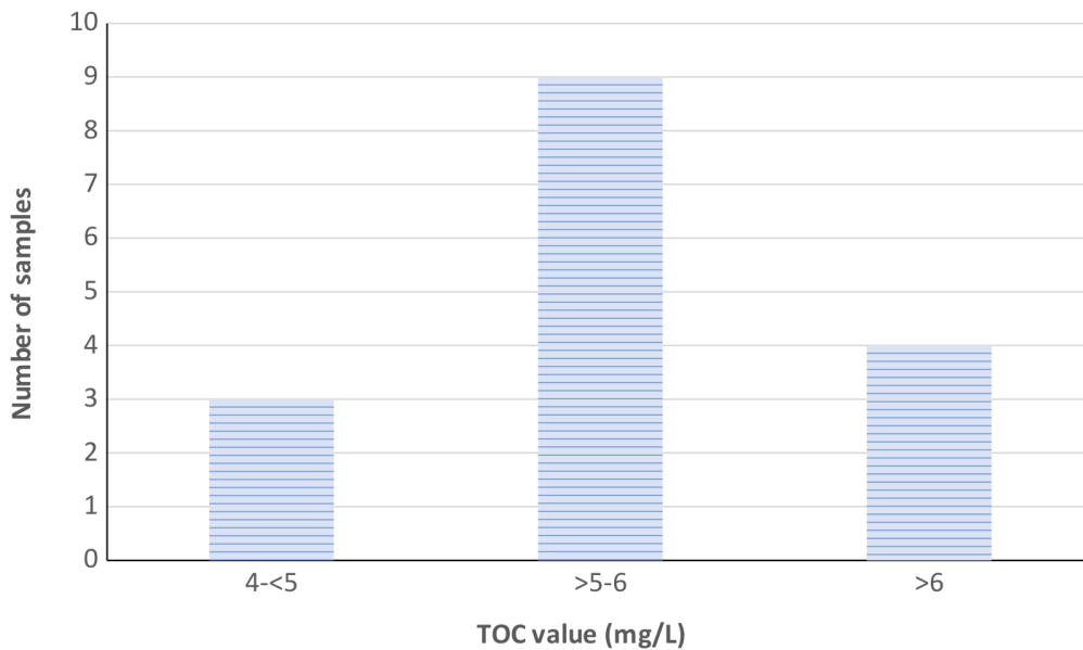
FIGURE 6. TOC value of groundwater in the study area.
