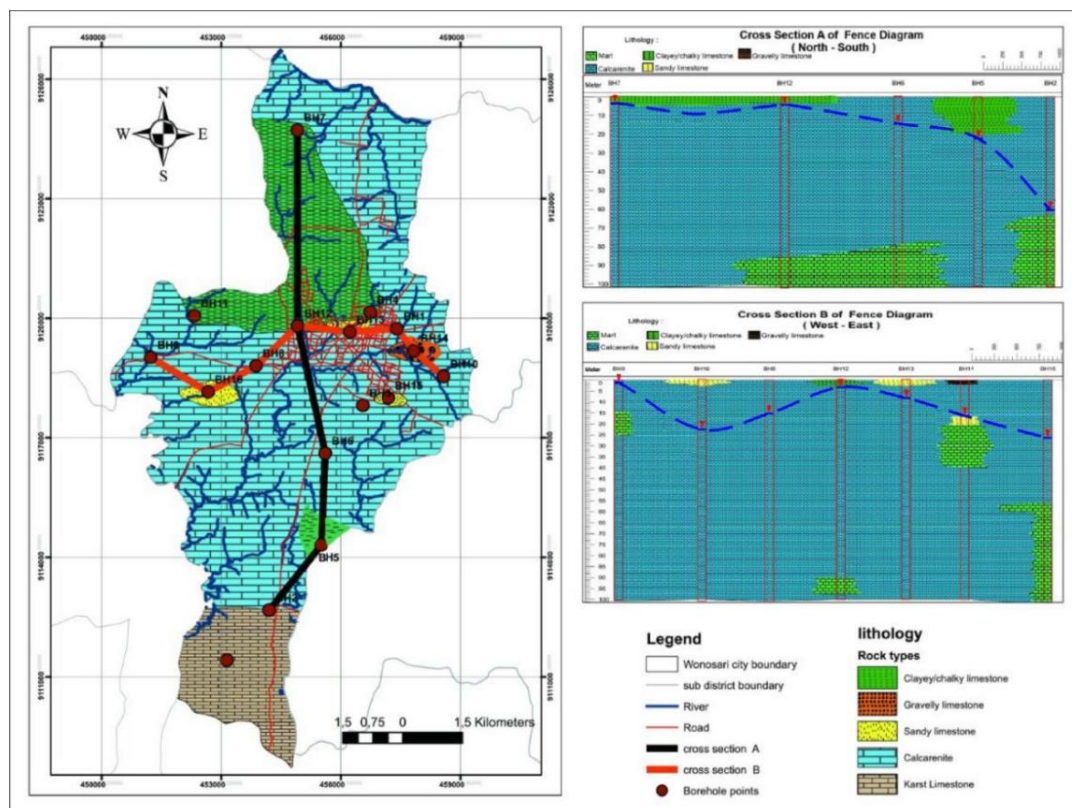
FIGURE 3. Surface and sub-surface lithology in the study area.
