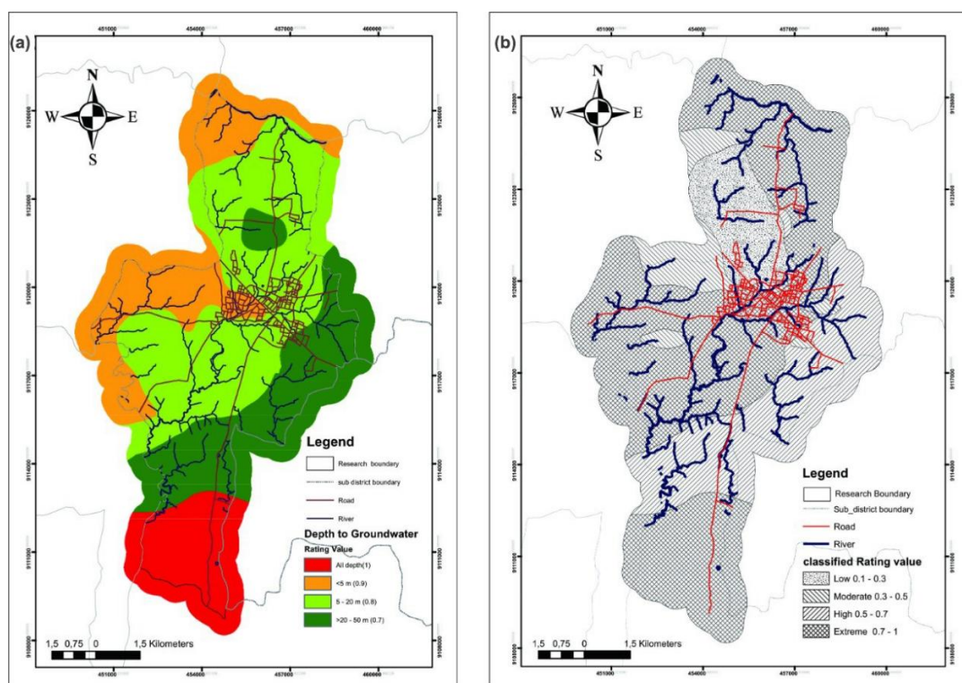
FIGURE 5. (a) GOD score of depth to groundwater parameter and (b) Groundwater vulnerability map based on GOD method in the study area.
