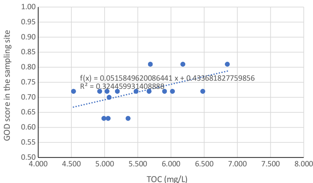
FIGURE 8. Relationship between TOC value in groundwater and GOD score in the sampling site.
