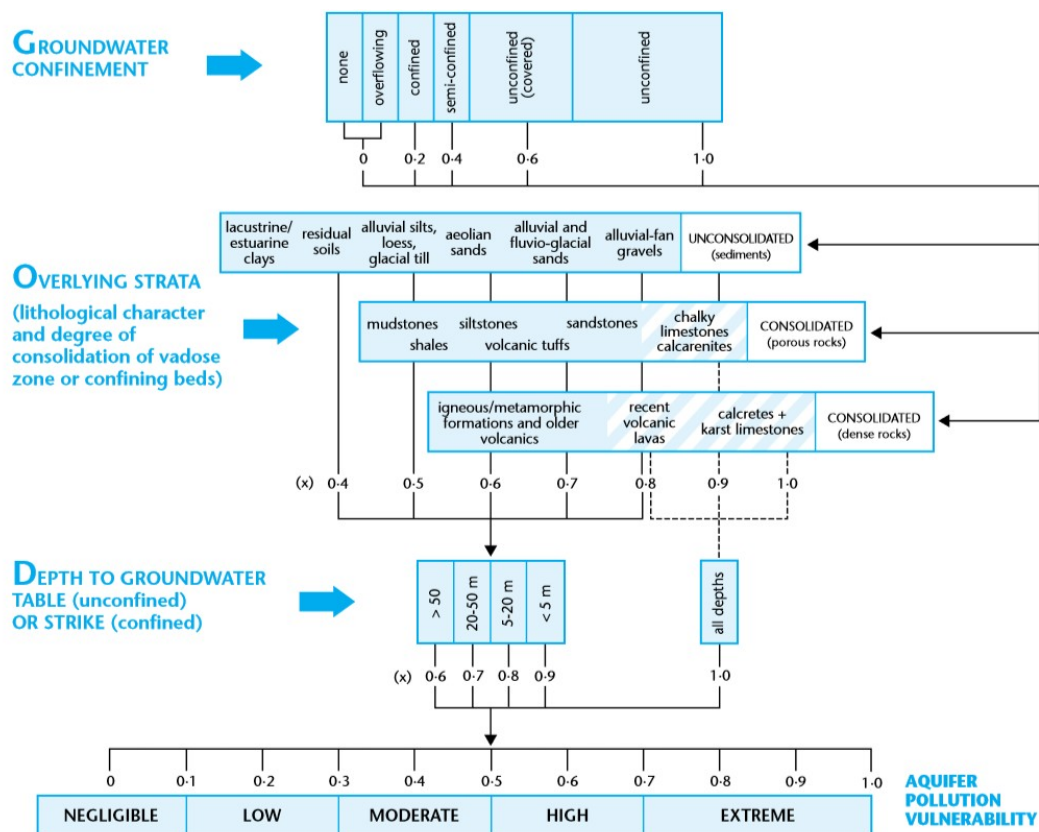
FIGURE 2. GOD method (Foster et al. , 2002).
