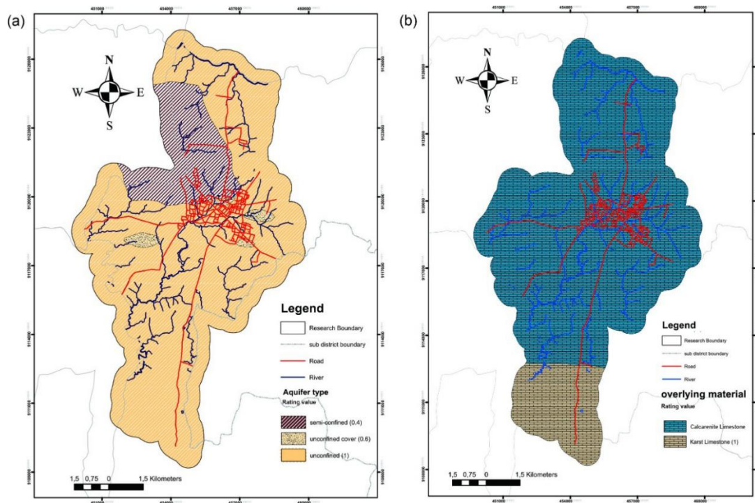
FIGURE 4. GOD score for (a) groundwater confinement and (b) overlying lithology in the study area.
