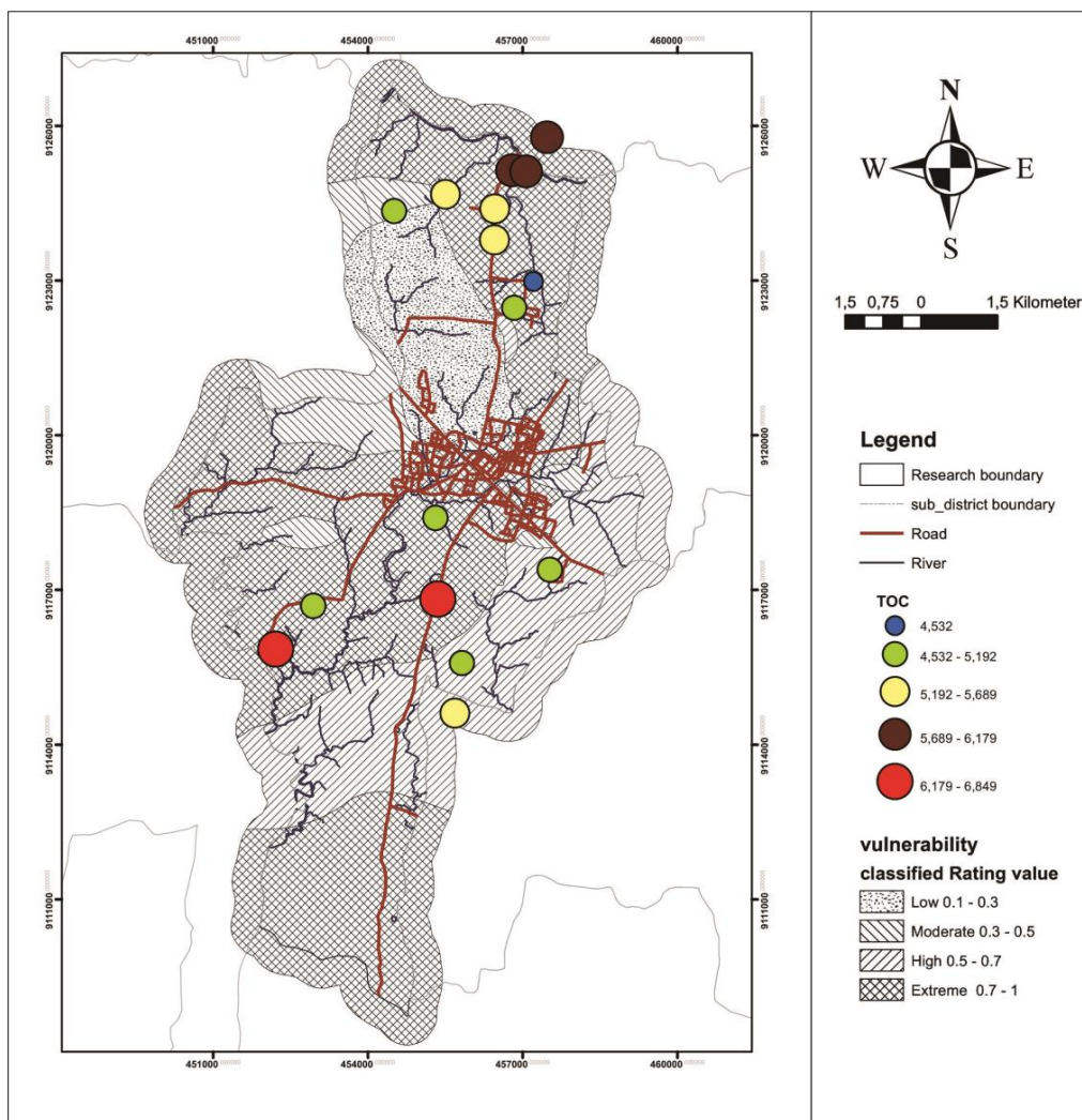
FIGURE 7. TOC value in groundwater versus GOD vulnerability class in the study area.
