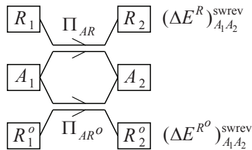
Figure 7. Schematic illustration of the processes used to define the temperature of a thermal reservoir.
