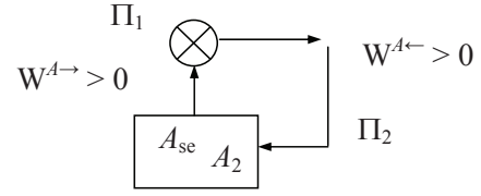
Figure 3. Schematic illustration of the proof of Theorem 1.
