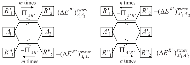
Figure 6. Illustration of the proof of Theorem 3, part b): sequence of processes (\Pi_A, \Pi_{A'}) , see text.
