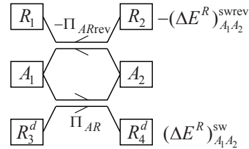
Figure 4. Illustration of the proof of Theorem 2: standard weight processes \Pi_{ARrev} (reversible) and \Pi_{AR} ; R^d is a duplicate of R ; see text.
