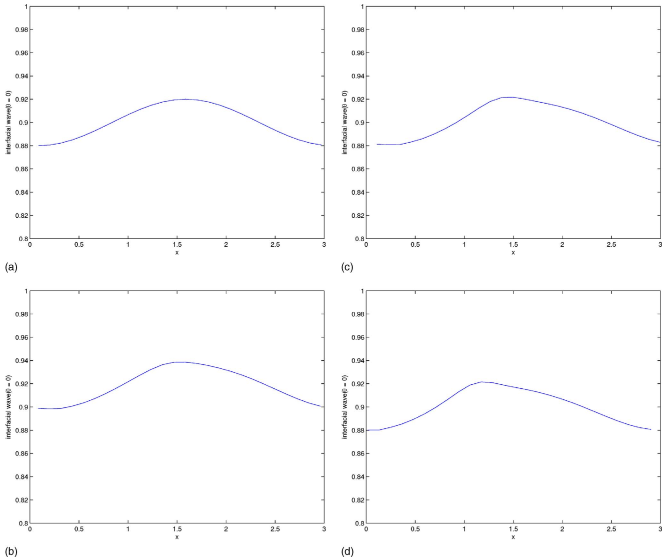
FIG. 9. (Color online) Movement of the wave at the interface (at top of the pipe) as a function of time. Concentric core at T=0 . Density difference between core and annulus. Pressure gradient over pipe. (a) After 0 time steps; (b) after 240 time steps; (c) after 690 time steps; and (d) after 900 time steps. C_1 = 10^{-3} , C_2 = 2 \cdot 10^{-3} , C_3 = 7 \cdot 10^0 , \Delta T = 10^{-4} , H_2^{(0)} = 0.1 , H_3^{(0)} = 0.8 , A = 0.02 , \epsilon = 0 , L = 3 , n_x = 26 , and n_t = 20 . The solid center is at rest according to the chosen reference system.
