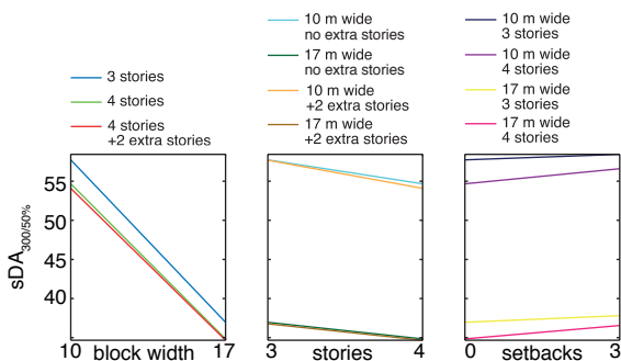
Figure 6 – Parameter-sensitivity plot: sDA 300
