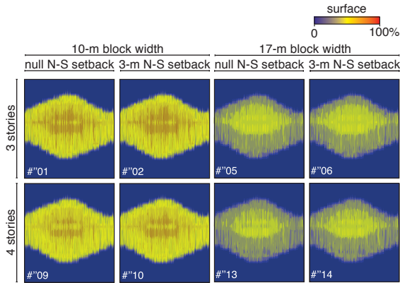
Figure 5 – False-color temporal maps: tDA 300
