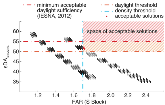
Figure 7 – Decision plot: selection of the acceptable solutions
