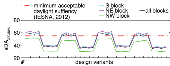
Figure 2 – Variant-performance plot: spatial Daylight Autonomy
