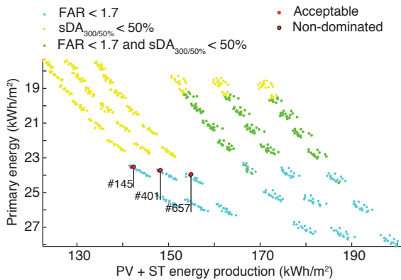
Figure 8 – Decision plot: selection of the optimal solutions
