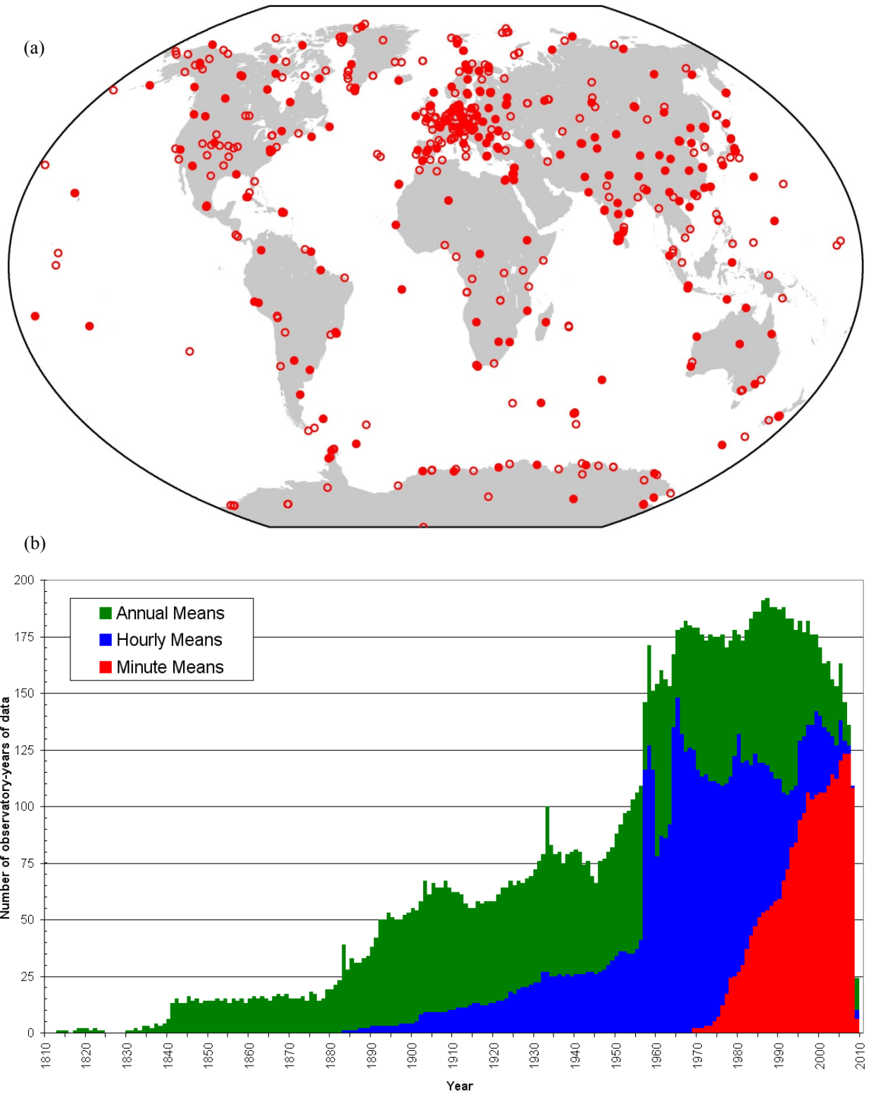
Fig. 7.7 (a) Locations of geomagnetic observatories worldwide, with data held in the Edinburgh WDC. Solid dots indicate operational observatories, open dots are sites that are currently closed (b) The number of data holdings at the World Data Centre (Edinburgh) for various time resolutions. (Copyright BGS/NERC)
