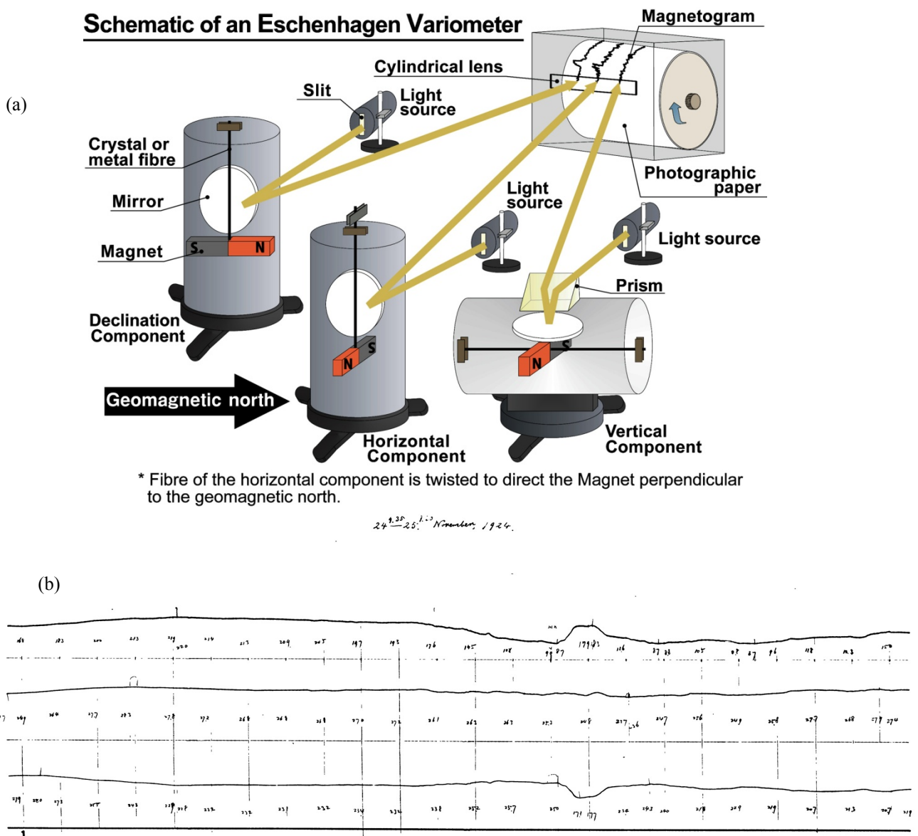
Fig. 7.2 (a) Schematic of an Eschenhagen type magnetic variometer (for details see Wienert, 1970) (b) Normal-run magnetogram recorded at Kakioka observatory on November 24, 1924. (Credit: WDC for Geomagnetism, Kyoto)
