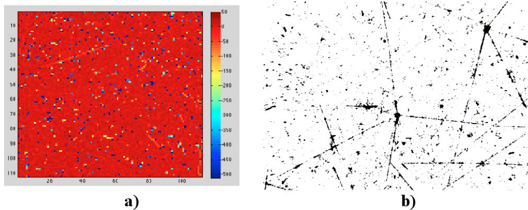
FIGURE 7. Low energy antiprotons annihilating on the detector surface. a) Mimotera pixel detector showing antiproton annihilation spots (dark blue), sporadic pion tracks are also visible (rare cases when pion was travelling along the detector's active volume). b) A developed and scanned nuclear emulsion after in-vacuum direct exposure to low energy antiprotons.
