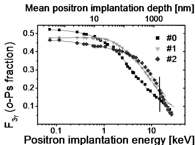
FIGURE 3. Fraction of implanted positrons annihilating via 3 gamma as ortho-positronium. Modified from [16]. Curves #0, #1 and #2 correspond to nanochannel diameter of 4-7 nm, 8-12 nm and 8-14 nm respectively.
