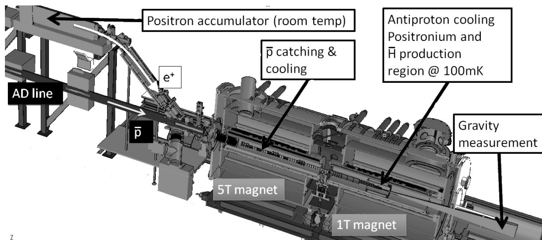
FIGURE 5. A 3D cut-open view of the full AEGIS apparatus at the CERN Antiproton Decelerator. During the first commissioning run the 1T magnet, the Moiré deflectometer and the positron transfer line were not present.
