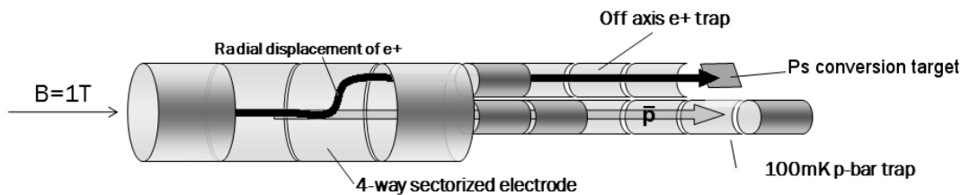
FIGURE 2. Schematic of the 1 T antihydrogen production trap system in AEGIS. The positron cloud is loaded into a high voltage off-axis trap using an autoresonance technique whereas antiprotons are transferred along the axis to the ultracold trap.
