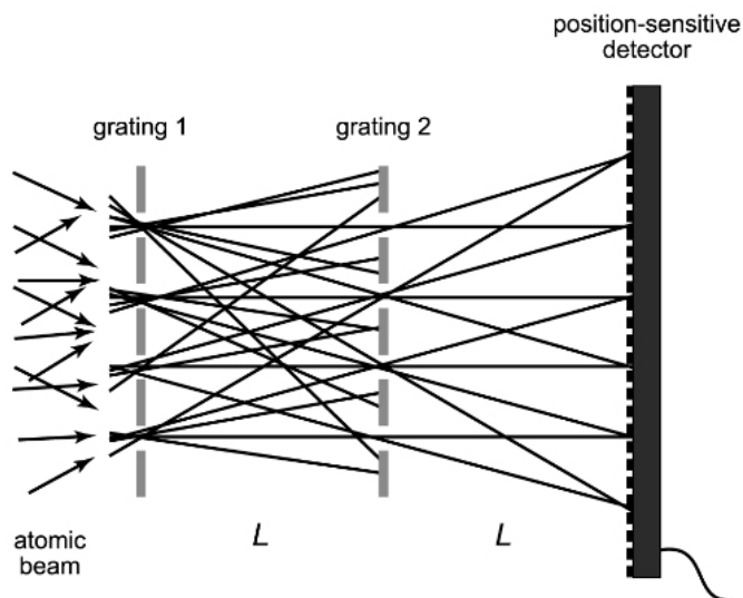
FIGURE 4. Schematic of the Moiré deflectometer in AEgIS with position sensitive detector instead of the third grating. With permission from [6].
