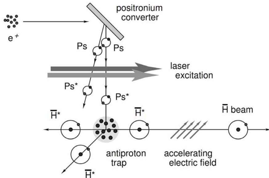
FIGURE 1. Schematic of pulsed antihydrogen production in AEGIS. With permission from [6].
