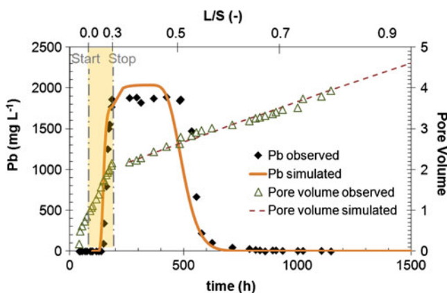
Fig. 4 Pb concentrations in the eluates and flushed pore volumes (observed and simulated) for column 2 (3 mmol kg -1 EDTA solution)
