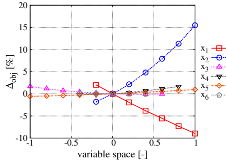
Fig. 10 Sensitivity analysis of design variables for the DTMB 5415 optimization
