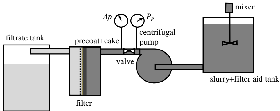
Fig. 1 - Layout for filtration with variable pressure due to centrifugal pump. The body-feed was simulated by premixed slurry with filter aid in the feed-tank
