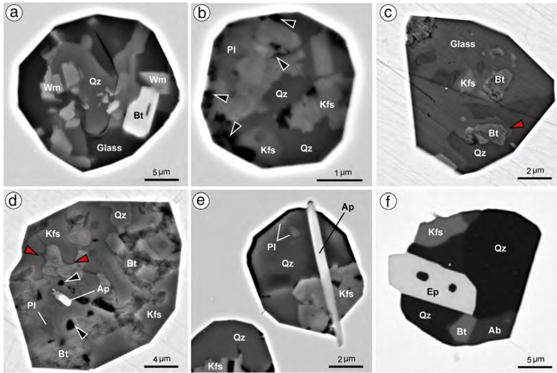
Fig. 6. SEM backscattered image of nanogranites . a) fully crystallized nanogranite in Ronda metatexites. b) nanogranite from the same location of (a) showing internal porosity (black arrows). c) partially crystallized inclusion, Kerala Khondalite Belt. Glass is still present, forming microstructures that are clear precursor of pseudomorphs after melt (red arrow). d) fully crystallized nanogranite with internal porosity (black arrow) from the same location of (c). Red arrow: sub-micrometric melt pseudomorphs of possible plagioclase. From (Cesare et al., 2009a). e) and f) nanogranites with trapped accessory phases indenting the inclusion walls. Samples from Ronda metatexites (e) and from the Orlica-Śnieżnik Dome in the Bohemian Massif (f).
