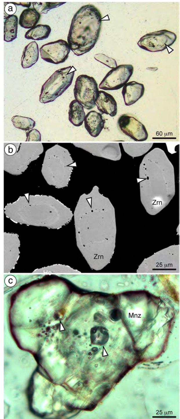
Fig. 12. a) plane-polarized photomicrograph of zircon crystals separated from a metapelitic enclave in the dacite at El Hoyazo. b) SEM backscattered image of a detail of the same separate. A very thin, BSE-bright annulus containing \mu\text{m} -sized glassy inclusions (arrows) separates inherited cores from euhedral overgrowths, grown in the presence of melt. c) Cluster of primary glassy inclusions (arrows) with shrinkage bubble at the core of a monazite crystal from Mazarrón. From Cesare (2008).
