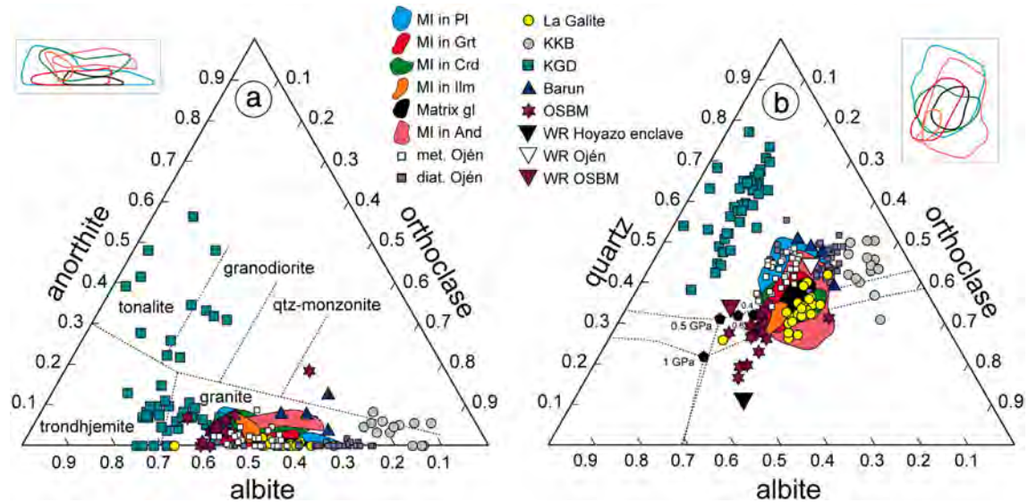
Fig. 13. Pseudoternary diagrams showing the wt.% normative An, Qz, Or and Ab compositions of all analyzed melt inclusions and matrix glasses in anatexic enclaves, and melt inclusions in migmatites and granulites. a) An–Or–Ab, with fields for granite, quartz–monzonite, granodiorite, trondhjemitic and tonalite after Barker (1979); b) Qz–Or–Ab, including equilibria data (cotectic lines, stippled, and eutectic compositions at 0.5 and 1.0 Gpa and a_{\text{H}_2\text{O}} = 1, 0.6 and 0.4 ) for the haplogranite system. Colored lines to the upper right of each triangular diagram show both the entire contours of, and spatial relationships among the solid colored fields in the diagram. Met = metatexites; diat = diatexites; KKB = Kerala Khondalite Belt; KGD = Kali Gandaki; and OSBM = Orlica–Śnieżnik Bohemian Massif.
