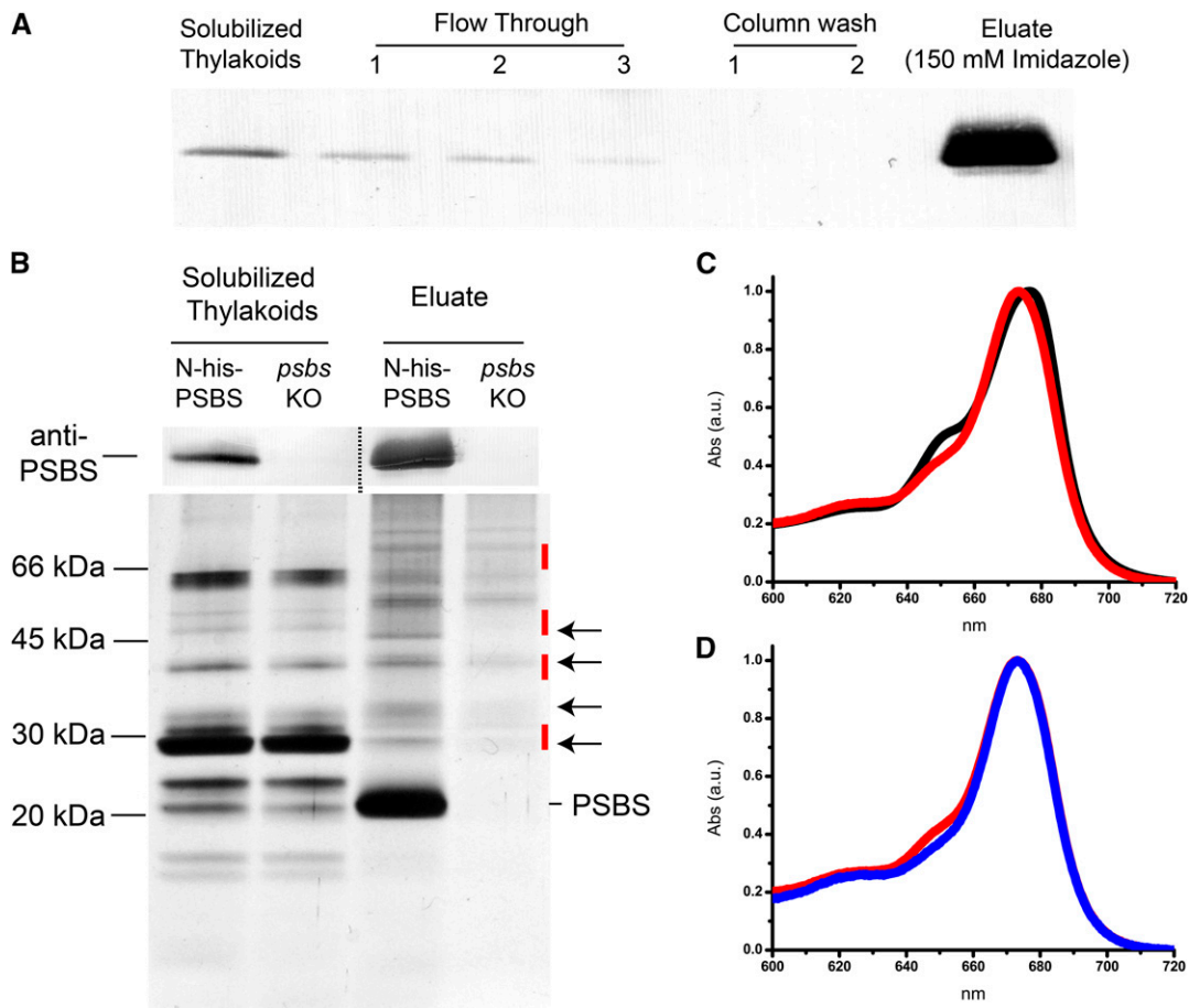
Figure 2. N-His-PSBS purification by affinity chromatography. A, Immunoblotting with anti-His-tag antibody on different purification fractions obtained from affinity chromatography of N-His-PSBS line 2 thylakoids. Fractions corresponding to starting material (solubilized thylakoids), flow through, column washes, and eluate with 150 mM imidazole are shown. B, PSBS immunodetection (top) and SDS-PAGE profile (bottom) of solubilized thylakoids and eluate with 150 mM imidazole from N-His-PSBS and psbs KO samples. Arrows indicate the main profile differences in N-His-PSBS and psbs KO eluates. Red segments indicate the gel regions where the proteins identified in Table II should be localized. One microgram of Chl was loaded for solubilized thylakoids and flow through in both A and B. For chromatography eluates, a volume corresponding to 15 (immunoblotting) and 130 (SDS-PAGE) \mu g of Chl in starting thylakoids was loaded. C, Absorption spectra of solubilized thylakoids (black) and N-His-PSBS eluate (red). D, Absorption spectra of eluates from N-His-PSBS (red) and psbs KO (blue). Spectra were normalized to the maximum of the red absorption band. a.u., Arbitrary units.
