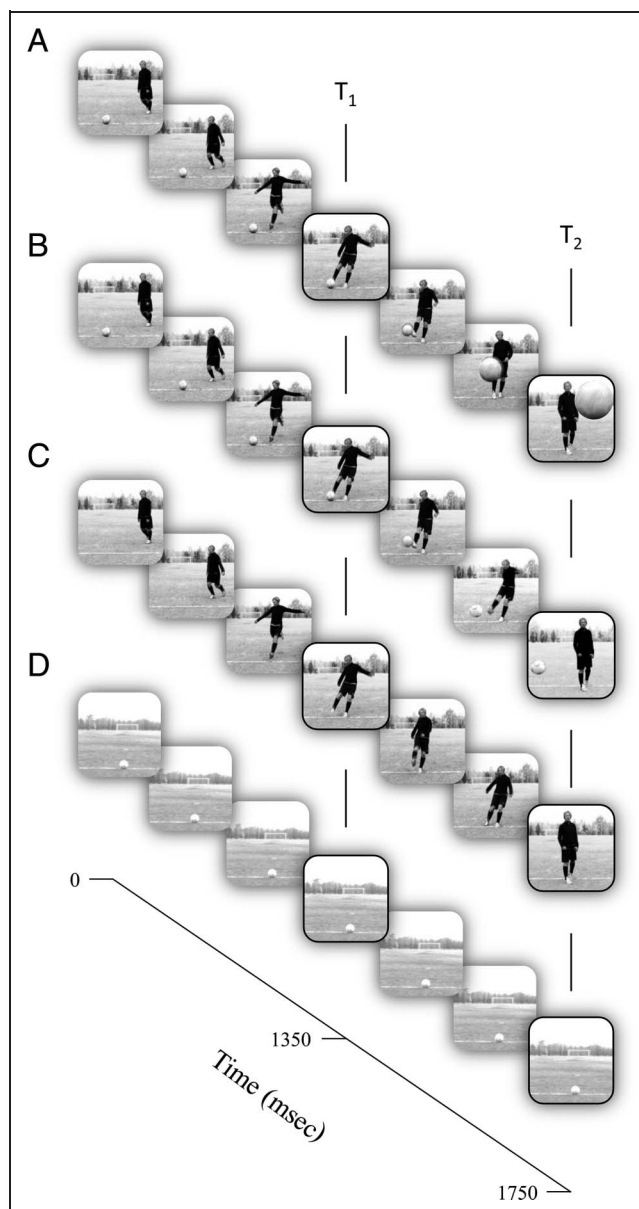
Figure 1. Sequence of events for each condition: (A) Central kick, (B) lateral kick, (C) mimicked kick, and (D) ball. The vertical lines denote the time points when single TMS pulses were delivered: at T_1 (when the player's foot made contact with the ball) and at T_2 (the end of the video clip).
