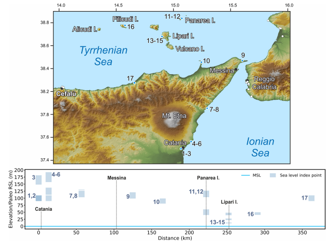
Figure 34. MIS5 sea-level data for Sicily, Sector 4 (Italy). Upper panel: map of sites. Red dots are sites in the region of interest, and white dots are other sites within the western Mediterranean compilation. The topography has been obtained from the SRTM void-filled DEM (Farr et al., 2007, NASA dataset). Lower panel: distance/elevation graph, counterclockwise from Catania to Cefalù. Sites list: 1: Catania (RSL ID 849); 2: Catania (II) (RSL ID 850); 3: Catania (III) (RSL ID 851); 4: Aci Trezza (RSL ID 846); 5: Aci Trezza (II) (RSL ID 847); 6: Aci Trezza (III) (RSL ID 848); 7: Taormina (II) (RSL ID 3626); 8: Taormina (RSL ID 903); 9: Capo Peloro (RSL ID 902); 10: Milazzo (RSL ID 921); 11: Panarea (RSL ID 917); 12: Panarea (II) (RSL ID 918); 13: Lipari (I) (RSL ID 909); 14: Lipari (II) (RSL ID 910); 15: Lipari (III) (RSL ID 911); 16: Filicudi (RSL ID 914); 17: Sant'Agata di Militello (RSL ID 924).
