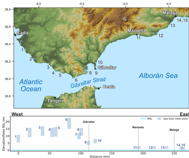
Figure 9. MIS 5 sea-level data for Andalusia (Spain). Upper panel: map of sites. Red dots are sites in the region of interest, and white dots are other sites within the western Mediterranean compilation. The topography has been obtained from the Shuttle Radar Topography Mission (SRTM) void-filled digital elevation model (DEM) (Farr et al., 2007, NASA dataset). Lower panel: distance/elevation graph from west (left) to east (right). Sites list: 1: Torre del Puerco (RSL ID 765); 2: Conil-Trafalgar (RSL ID 764); 3: Zahara (RSL ID 763); 4: Cabo Gracia (RSL ID 762); 5: Bolonia – Punta Paloma (RSL ID 761); 6: Tarifa (RSL ID 760); 7: Algeciras 1 (RSL ID 758); 8: Algeciras 2 (RSL ID 759); 9: Gibraltar (RSL ID 757); 10: La Linea (RSL ID 756); 11: Marbella (RSL ID 755); 12: Fuengirola (RSL ID 754); 13: Torremolinos (RSL ID 753); 14: El Candado (RSL ID 752); 15: Cerro Juan (RSL ID 4001).
