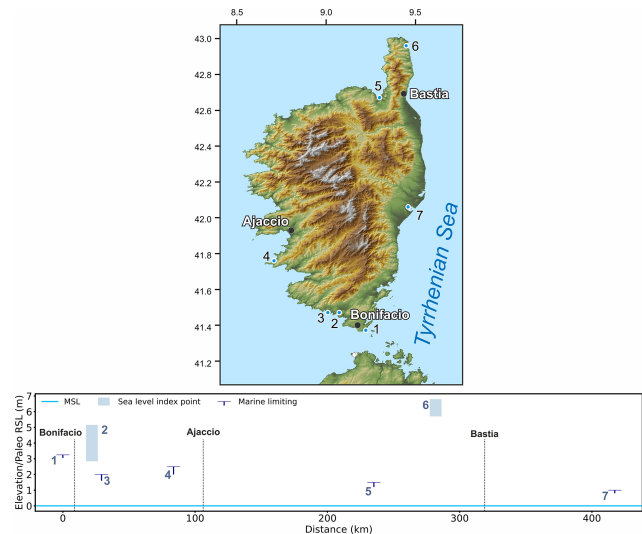
Figure 29. MIS 5 sea-level data for Corsica (France). Upper panel: map of sites. The topography has been obtained from the SRTM void-filled DEM (Farr et al., 2007, NASA dataset). Lower panel: distance/elevation graph, clockwise around the island starting from the southernmost point. Sites list: 1: Piantarella (RSL ID 277); 2: Figari (RSL ID 321); 3: Arbitru (RSL ID 323); 4: Ajaccio Gulf Capo Moru (RSL ID 303); 5: St Florent (RSL ID 299); 6: Macinaccio Tamarone (RSL ID 931); 7: Urbino (RSL ID 322).
