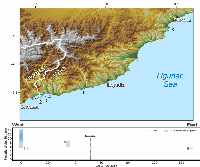
Figure 15. MIS 5 sea-level data for Liguria (Italy). Upper panel: map of sites. The topography has been obtained from the SRTM void-filled DEM (Farr et al., 2007, NASA dataset). Lower panel: distance/elevation graph, from west (left) to east (right). Sites list: 1: Ex Casino (RSL ID 240); 2: Barma Grande (RSL ID 233); 3: Bausu da Ture (RSL ID 239); 4: Grotta del Principe (RSL ID 237); 5: Madonna dell'Arma (RSL ID 242); 6: Grotta Marina di Bergeggi (RSL ID 246).
