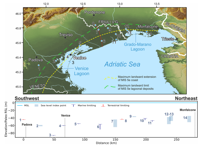
Figure 28. MIS 5 sea-level data for Veneto and Friuli Venezia Giulia (Italy). Upper panel: map of sites. The topography has been obtained from the SRTM void-filled DEM (Farr et al., 2007, NASA dataset). Lower panel: distance/elevation graph, from southwest (left) to northeast (right). The lines depicting the innermost position of the coastline and of the lagoon deposits of MIS 5e are modified after Antonioli et al. (2009). Sites list: 1: Ca' Borille Core (RSL ID 1306); 2: Valle Averte Core CARG 11 (RSL ID 1304); 3: Malamocco Core (RSL ID 1305); 4: VE-1 Core Venezia1 (RSL ID 1303); 5: Portegrandi Core CARG12 (RSL ID 1302); 6: TdM Torre di Mosto Core (RSL ID 1295); 7: PRA Belfiore Core (RSL ID 793); 8: AZX Azzano Core (RSL ID 1301); 9: CNC4 Concordia Sagittaria Core (RSL ID 1289); 10: LUG Lugugnana Core (RSL ID 1294); 11: VV Valle Vecchia Core (RSL ID 1293); 12: Piancada Piancada town (RSL ID 1291); 13: PNC1 Piancada Core (RSL ID 1292); 14: BLG1, Beligna Core (RSL ID 1290). The red line connecting points 6–8 represents the cross section of Fig. 27.
