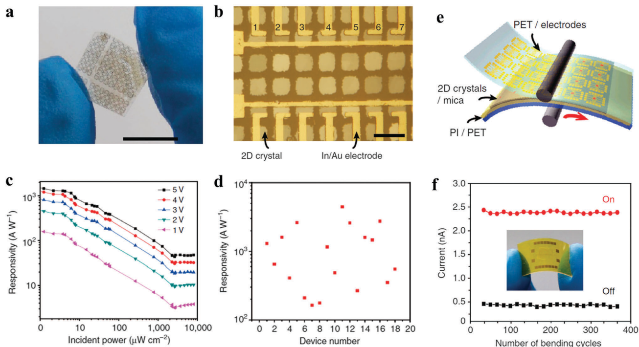
Fig. 11 (a) Photograph and (b) optical microscope image of \alpha - \text{In}_2\text{Se}_3 photodetector arrays on mica substrate. Scale bars in (a) and (b) are 1 cm and 20 \mu\text{m} , respectively. (c) Dependence of R on illumination intensities and voltage bias. (d) Statistic distribution of R \alpha - \text{In}_2\text{Se}_3 photodetectors. (e) Schematic of device packaging. (f) Current as a function of bending cycles (10 mm radius) of the packaged \alpha - \text{In}_2\text{Se}_3 photodetector devices at a bias voltage of 5 V. The inset shows the photograph of packaged device; (a–f) are reproduced from ref. 163 with permission from Macmillan Publishers Ltd, Copyright 2015.
