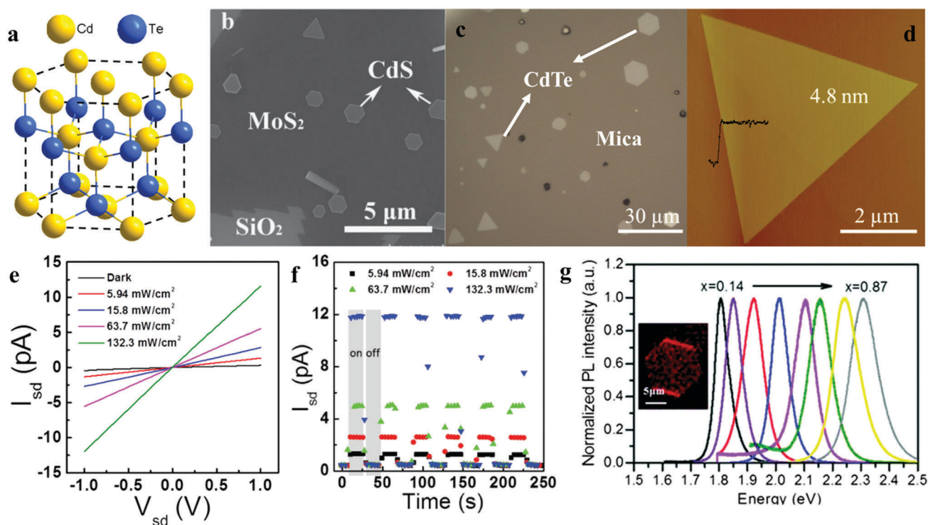
Fig. 20 (a) Schematic illustration of CdX (X = S, Se, Te) with a wurtzite structure using CdTe as an example. (b) SEM image of epitaxial CdS nanosheets on a monolayer MoS 2 . (c) Optical image of epitaxial CdTe nanosheets on a mica substrate. (d) AFM image of a typical CdTe nanosheet with thickness of 4.8 nm. (e and f) I_{DS} - V_{DS} output curves and time-dependent photoresponse of 2D CdTe photodetector under 473 nm laser illumination. (g) Normalized PL spectra of CdS 1-x Se x alloy nanosheets with different compositions; (a and c-f) are reproduced from ref. 286 with permission from John Wiley & Sons, Inc., Copyright 2017, (b) is reproduced from ref. 285 with permission from John Wiley & Sons, Inc., Copyright 2016, and (g) is reproduced from ref. 287 with permission from the Royal Society of Chemistry, Copyright 2017.
