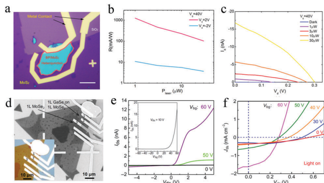
Fig. 23 (a) Optical image of the fabricated device. The dark purple region is monolayer MoS 2 , while the blue flake is few-layer black phosphorus. The light purple region is SiO 2 . Scale bar, 10 μm. (b) Photodetection responsivity ( R ) calculated as a function of incident power. (c) I DS as a function of V DS under various laser powers. The I sc and V oc can be obtained from the intercepts of the curves on I DS and V DS axes. (d) SEM image of a device made on a 1L MoSe 2 partially covered by 1L GaSe domains. Electrodes 1 and 2 were made on the GaSe/MoSe 2 vdW heterostructure region, whereas electrode 3 was made on a bare 1L MoSe 2 region. Inset shows the corresponding optical micrograph. (e) I DS – V DS curves across the p(GaSe)–n(MoSe 2 ) heterojunction (measured using electrodes 2 and 3) at different back-gate voltages (without illumination). The inset shows the I DS – V GS curve (with V DS fixed at 10 V) across the heterojunction. (f) J DS – V DS curves with white light illumination across the heterojunction at different back-gate voltages; (a–c) are reproduced from ref. 302 with permission from American Chemical Society, Copyright 2014 and (d–f) are reproduced from ref. 308 with permission from AAAS, Copyright 2016.
