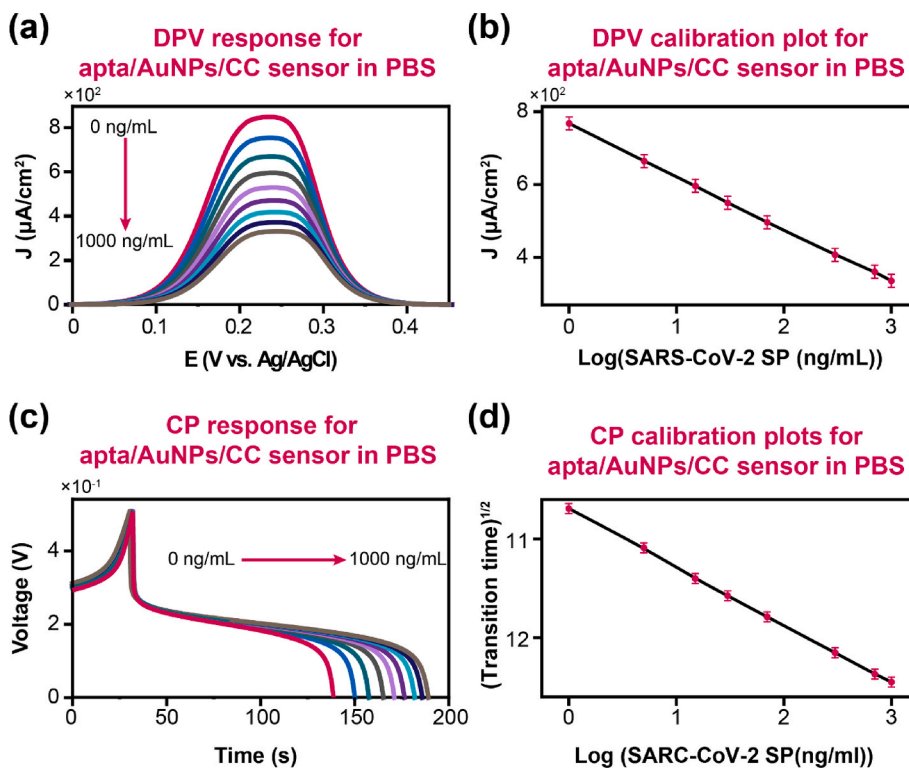
Fig. 5. (a,c) DPV and CP responses obtained at the apta/AuNPs/CC sensor incubated in PBS solutions containing different concentrations of SARS-CoV-2 SP (0, 2, 6, 20, 60, 200, 600, and 1000 ng/mL). (b,d) Calibration plots obtained using DPV and CP, respectively; they include error bars, obtained from three replicates. The star symbol refers to the responses obtained in the medium without SARS-CoV-2 SP. All measurements were performed in the solution containing [\text{Fe}(\text{CN})_6]^{3-/4-} redox probe.
