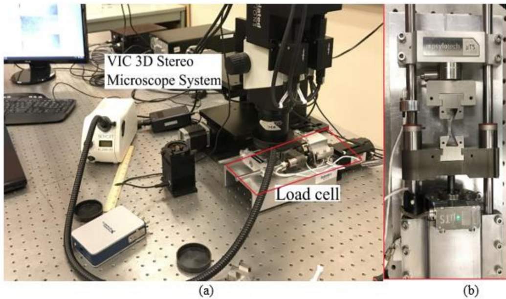
Figure A3. Experimental setup (a) for uniaxial tensile loading of RDD0, RDD45, RDD90 specimens using microscope Stereovision and micro-tensile test system (b) close view of micro-tensile test grip.
