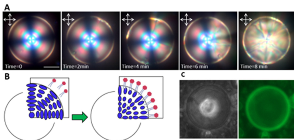
Figure 1. Reconfiguration of high-chirality LC droplets in the presence of DLPC amphiphiles. (A) Reflection mode POM images of reconfiguration dynamics in 30\text{ }\mu\text{m} high-chirality droplets in the presence of 0.5\text{ mM} DLPC. (B) Schematic of the planar to homeotropic ordering transition. (C) Bright-field and fluorescent image of adsorbed labeled DLPC amphiphiles on the chiral droplet's interface (scale bar = 20\text{ }\mu\text{m} ).
