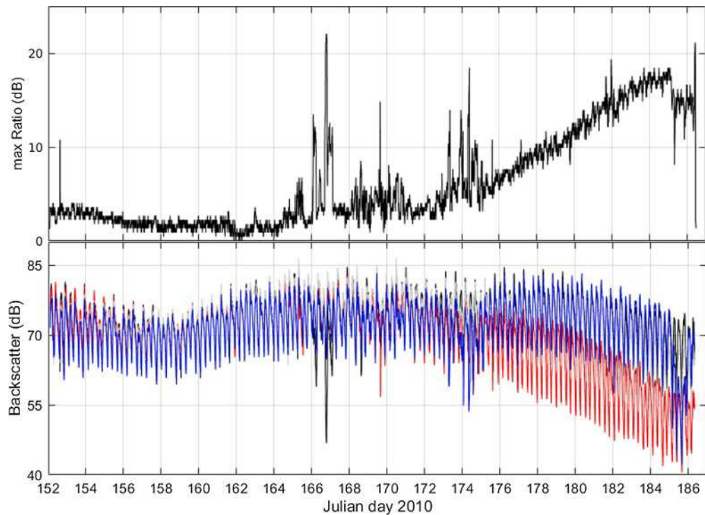
Figure 5: 35-day time series of cross-beam backscatter ratio (up) and the acoustic backscatter intensity (down) recorded by an upward-looking 1.2 MHz RDI ADCP (5th bin at about 1.5 m above the ADCP is shown) moored offshore the Belgian coast. Changes in the cross beam backscatter ratio, R_v , occurred from day 165 onward and from day 172 a gradual increase is observed. Superposed are quarter-diurnal variations in R_v of the order of 2–3 dB that result from the deposition of fine sediments during slack water and the subsequent erosion during increasing currents. The recovered ADCP was massively fouled by barnacles, tube building worms and hydrozoa
