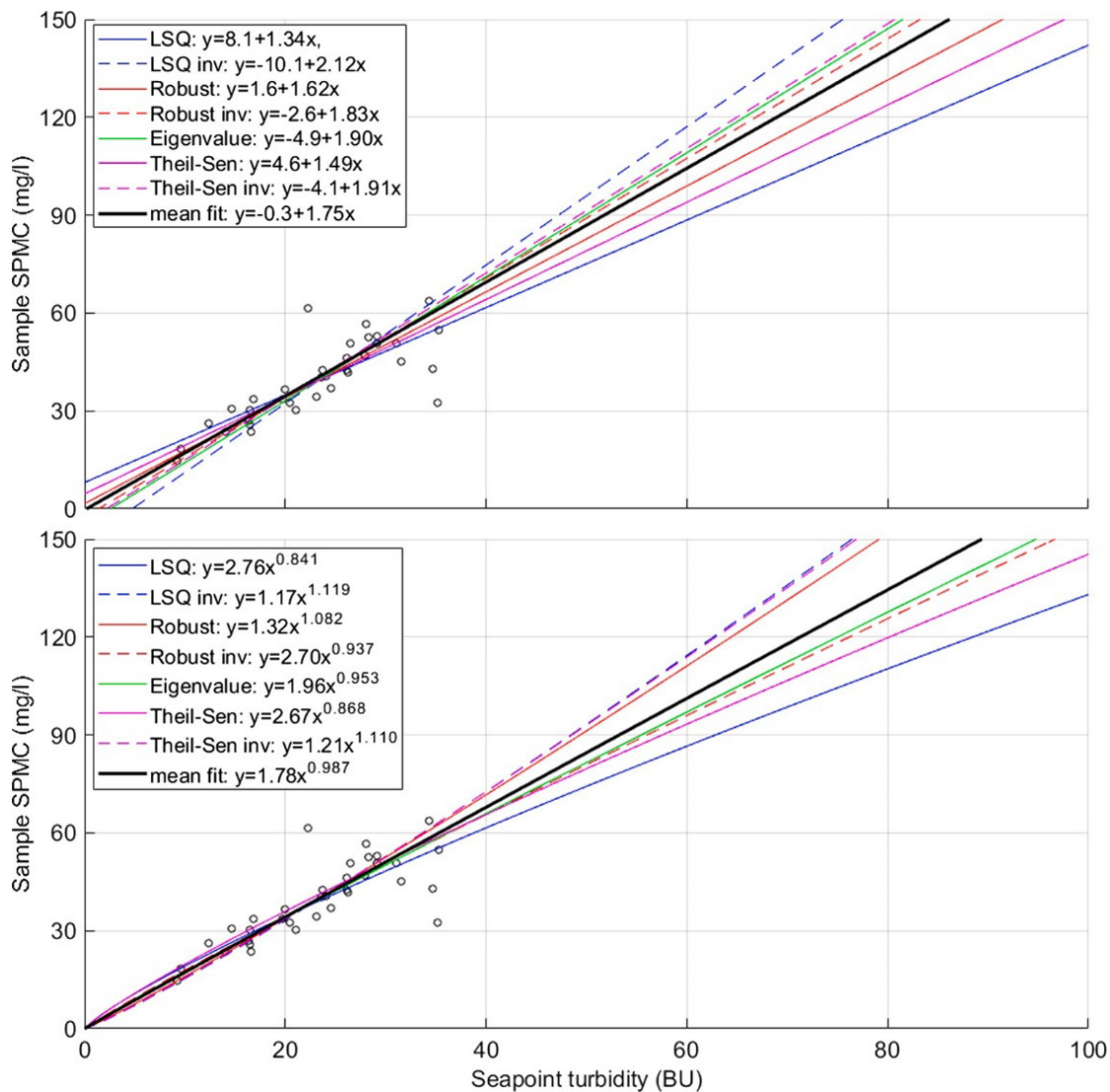
Figure 9: Relating sample SPMC to sensor output using different linear regression models for the actual and the log transformed data ( R^2 = 0.61 , 26 samples). The data have been collected in the Belgian nearshore area and consist of 26 sample SPMC and corresponding turbidity values from a Seapoint OBS. The solid lines correspond to the relationship BU = f(\text{sample SPMC}) and the dash lines to \text{sample SPMC} = f(BU) . The bold line is the mean of the 7 regressions and represents a baseline to show the variability of the different regression models (compare Sections 3.4.2 and 4.1.4).
