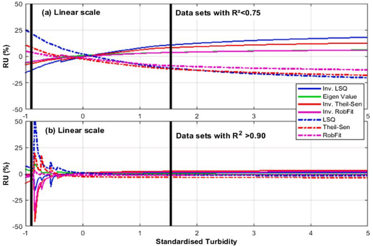
Figure 13: Regression model choice uncertainty (RU) for the different regression models as a function of standardized turbidity ( T_{z\text{-std}} ) for the linear scale. The examples show RU averaged over data sets with R^2 < 0.75 (upper panels) and R^2 > 0.90 (lower panels). The black lines represent the 10 and 90% percentiles of T_{z\text{-std}} averaged over all calibration data sets. Note the different limits in the ordinates of the left and the right panels.
