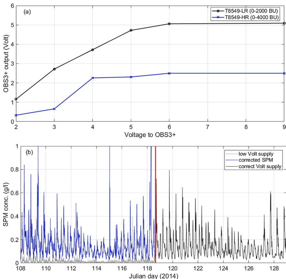
Figure 2: (a) Power provided by an external source to a OBS3+ (T8549) measuring in high and low range in a standard solution of 2000 AMCO Clear® equivalent BU. When the voltage drops
