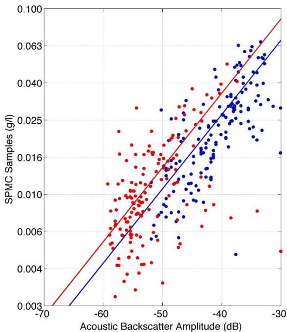
Figure 10: Direct calibration of a profiling acoustic sensor (Nortek AWAC) against sample SPMC in a moderately turbid environment ( < 100 mg/l) located at the mouth of the Seine estuary (red dots: surface samples, blue dots: bottom samples).
