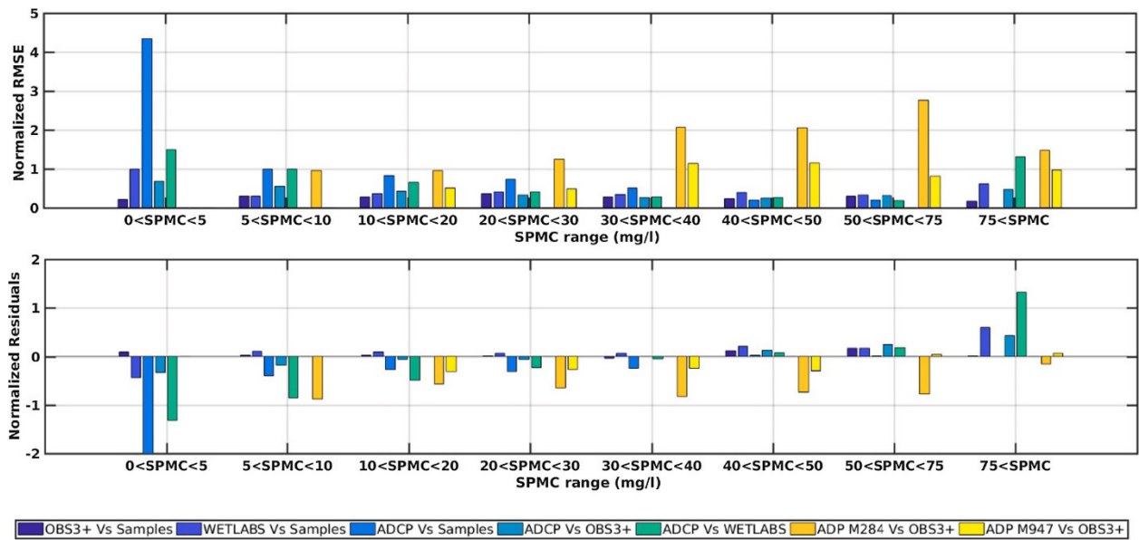
Figure 19: The model SPMC uncertainty (normalized RMSE and residuals) as a function of the reference SPMC (sample or sensor derived SPMC) and SPMC range (see the dataset shown in Figs. 10 and 11) for an acoustical and some optical backscatter sensors. The reference SPMC is from sample or OBS3+ derived SPMC.
