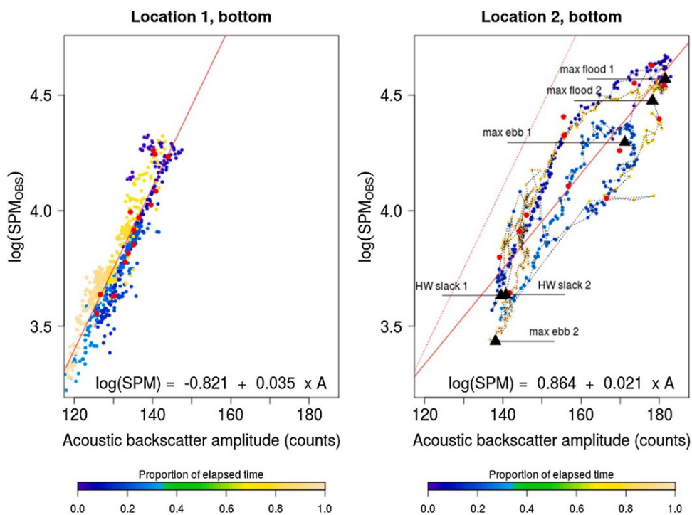
Figure 17: Relation between optical (YSI, type 6920 V2) and acoustical backscatter sensor (ADV (Nortek, 6 MHz) at a muddy (location 1) and a sandy bed site (location 2) located 1200 m apart in the main tidal channel of a brackish marsh located in the Scheldt estuary during 2 tidal cycles (Schwarz et al., 2017).
