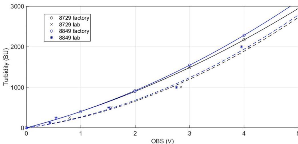
Figure 1: Factory and in lab sensor calibration of two OBS3+ (8729 and 8849). The laboratory calibration was done after 421 (8729) and 329 (8849) days of measurements in high turbid (SPMC > 1 g/l) sea water during the period 2014–2016. The solid lines are the 2nd order polynomial fittings provided by the factory, the dashed lines are the 2nd order fittings after recalibration.
