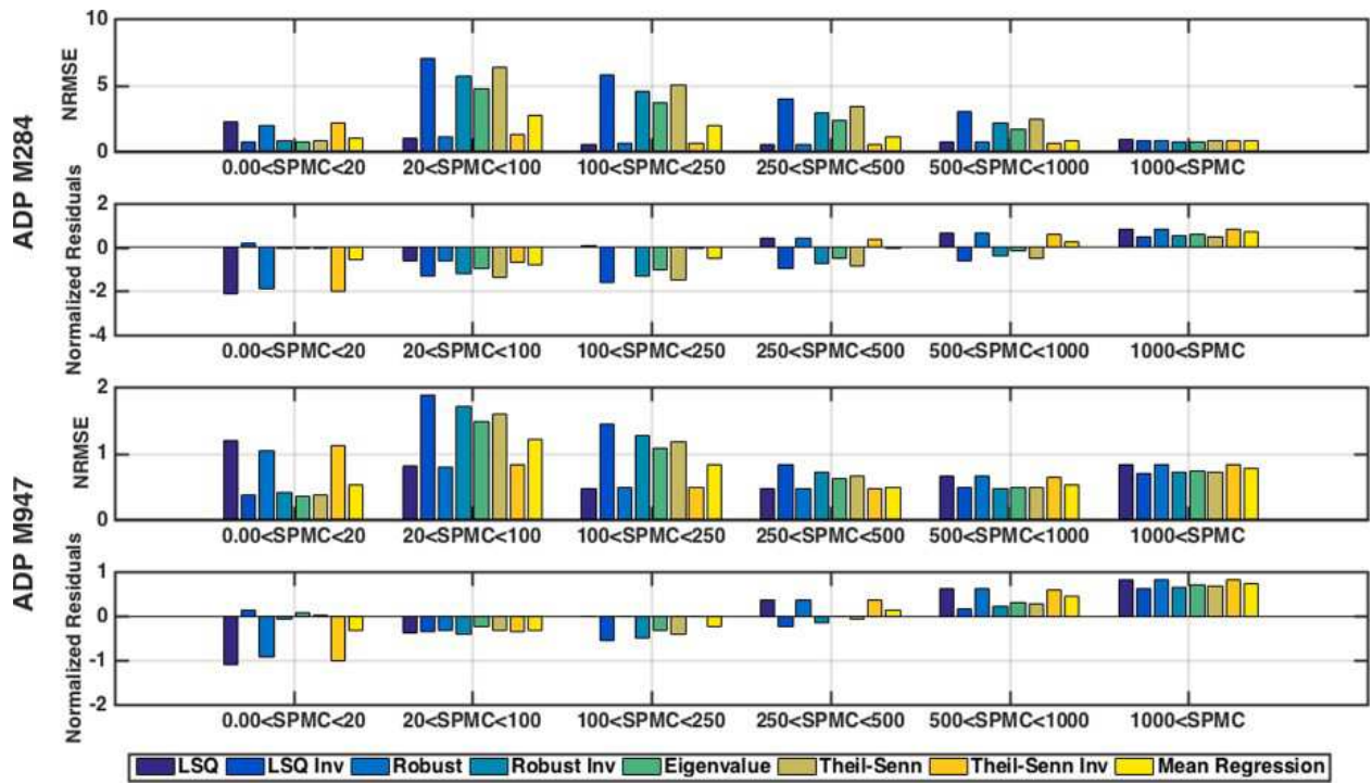
Figure 20: The model SPMC uncertainty for the ADP's of Fig. 11 expressed as normalized RMSE and normalized residual for different regression models and as a function SPMC. Negative residuals have a higher ADP-derived SPMC than the OBS-derived one.
