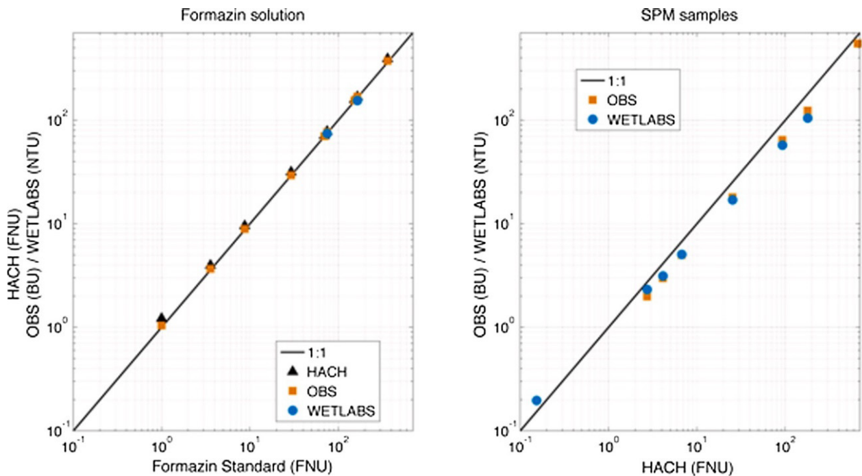
Figure 23: The performance of different sensors (side-scattering: Hach; backscattering: OBS3+ and Wetlabs) during sensor calibration with different formazine solutions (left) and as compared with natural SPM samples.
