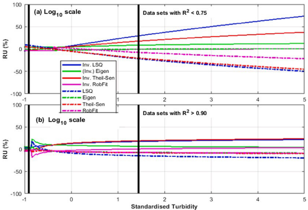
Figure 14: Idem Fig. 13 but now for the \log_{10} – transformed data.
