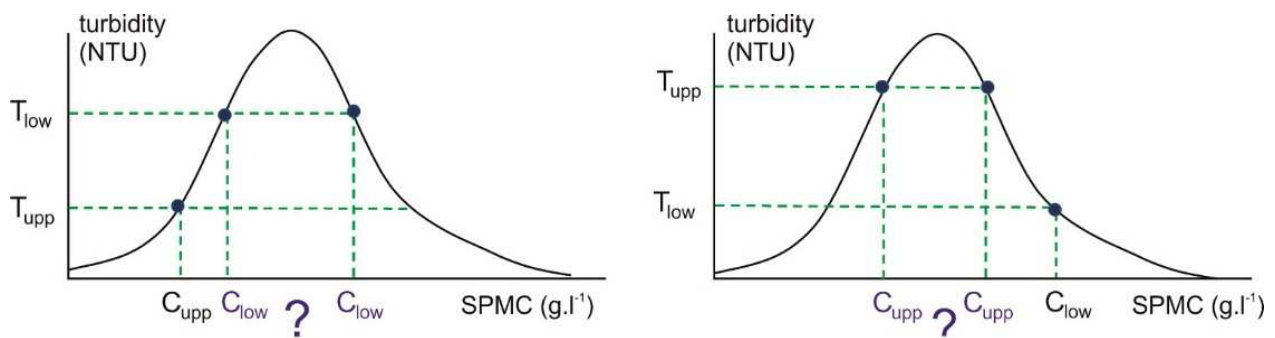
Figure 7: Typical bell-shaped backscatters curve of an OBS (Sottolichio et al., 2011), meaning that a given OBS output can correspond to two SPMC values. The figure shows how this ambiguity can be solved by using two superimposed sensors. Left: when the upper probe records lower turbidity than the lower probe, upper concentration is solved, but the lower remains unsolved. Right: when the upper probe records higher turbidity than the lower one, lower concentration is solved, but the higher remains ambiguous and unsolved.
