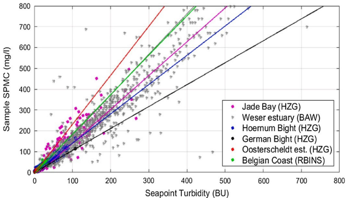
Figure 15: Sample SPMC as a function of Seapoint turbidity collected at various locations in the southern North Sea. The regression is calculated with the Eigenvalue model. The mean regressions are (SPMC = ax + b ): all data ( R^2 = 0.88 ; a = 1.53 , b = -1 ); Jade Bay ( R^2 = 0.83 ; a = 1.95 , b = -17 ), Weser estuary ( R^2 = 0.83 ; a = 1.62 , b = -21 ); Hoernum Bight ( R^2 = 0.95 ; a = 1.41 ,
