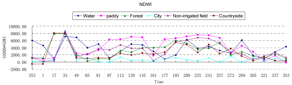
Fig. 3 Multi-temporal NDVI, EVI and NDWI profiles of the major land use types
