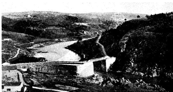
The Pinay Dam on the Loire River in southern France.
