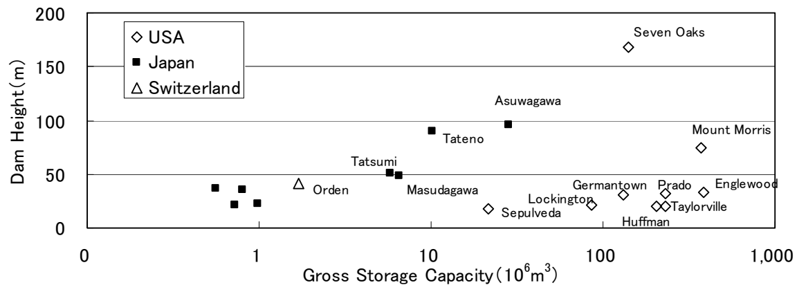
Figure 3 Gross storage capacity and dam height of flood retention ‘Dry dams’
