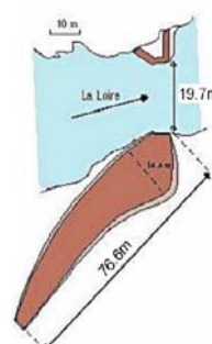
Figure 5 Pinay dam in Loire River in France completed in 1711
