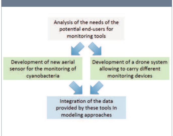
Figure 2. OSS-Cyano methodology
